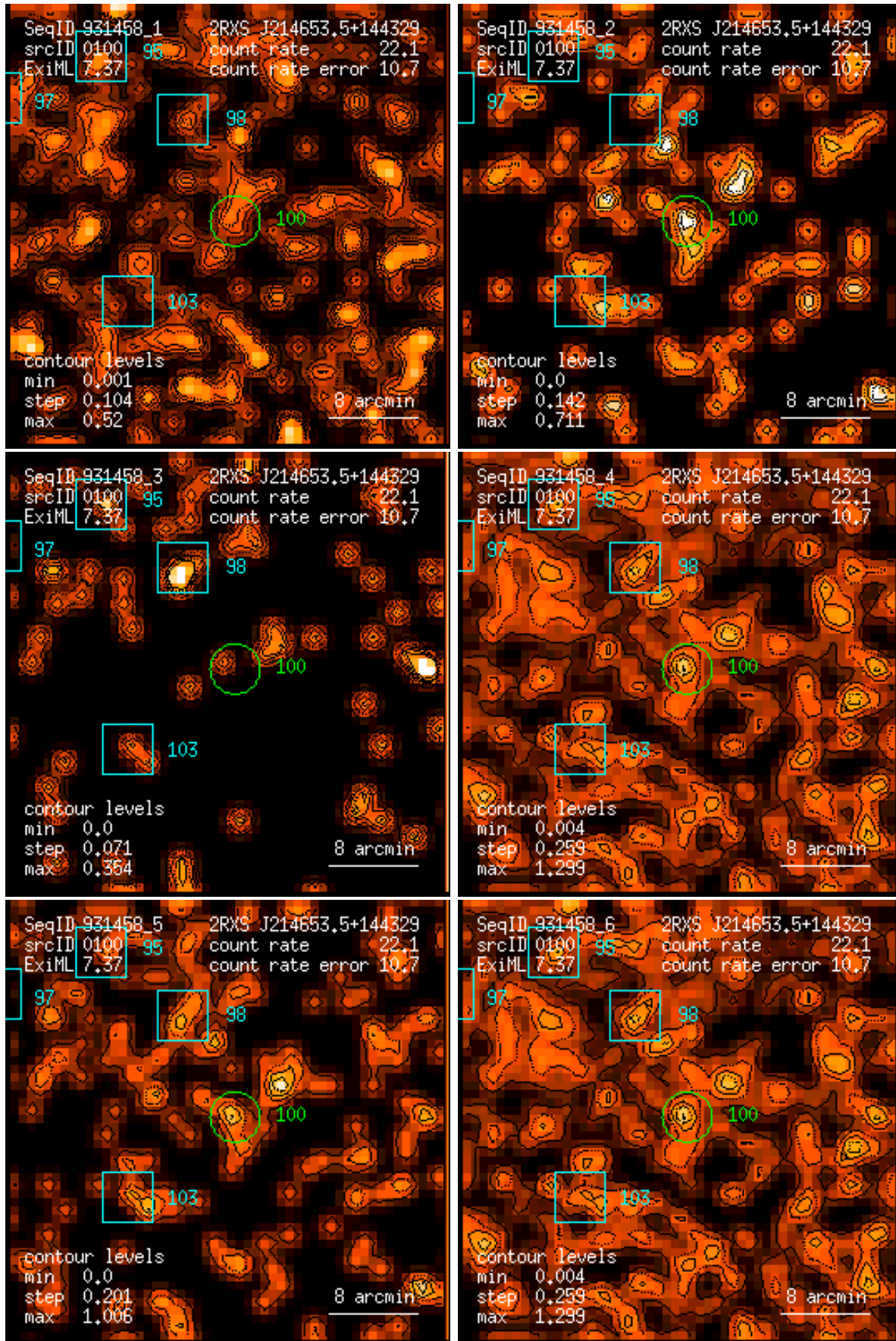
Figure 100: RASS 931458: detection 0100: band rate images, Gaussian filter: (1) PSPC channels 11 – 41, (2) 52 – 90, (3) 91 – 201, (4) 11 – 235, (5) 52 – 201, (6) 11 – 201. Broad band rates in counts/ks. Band rate contour levels in counts/ks/arcmin 2 .
