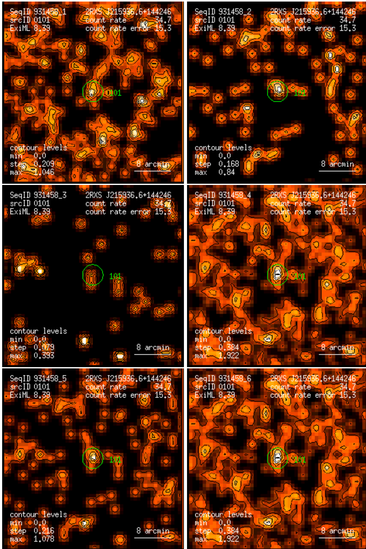
Figure 101: RASS 931458: detection 0101: band rate images, Gaussian filter: (1) PSPC channels 11 – 41, (2) 52 – 90, (3) 91 – 201, (4) 11 – 235, (5) 52 – 201, (6) 11 – 201. Broad band rates in counts/ks. Band rate contour levels in counts/ks/arcmin 2 .
