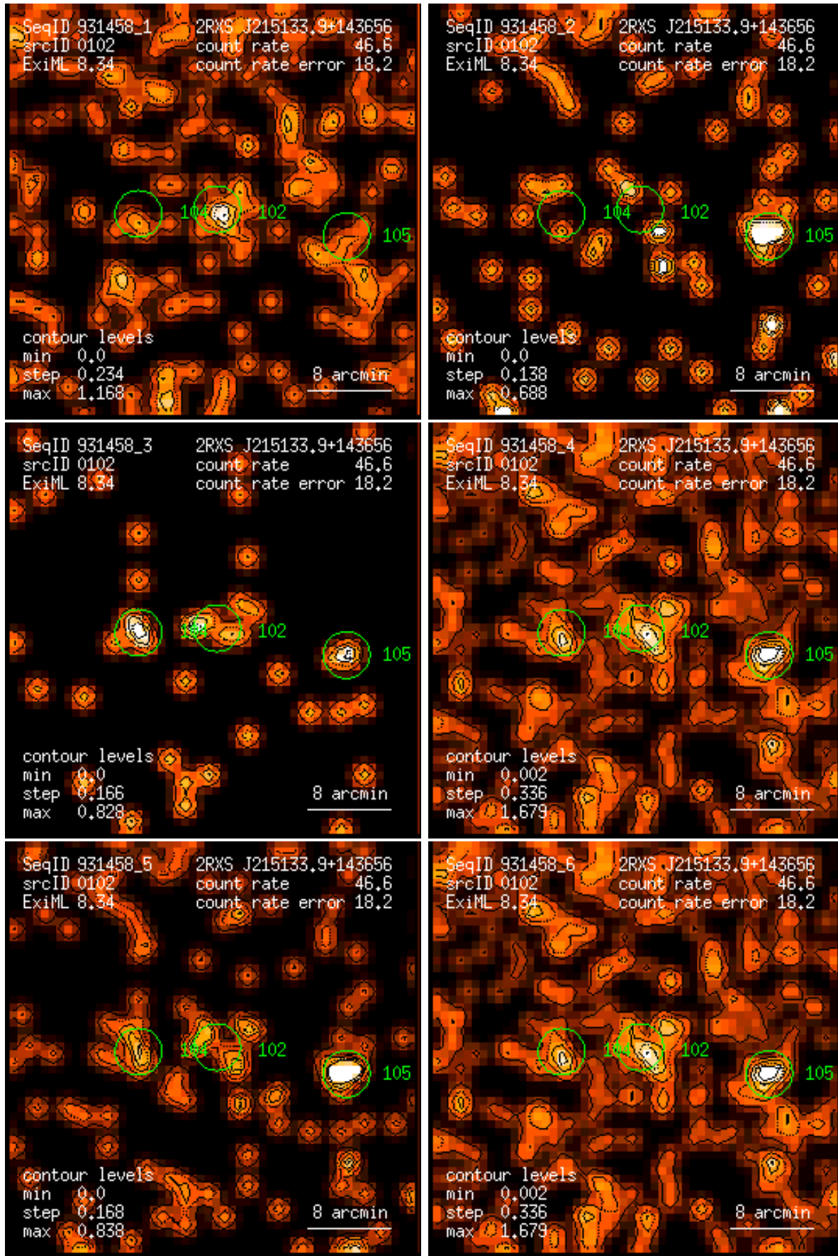
Figure 102: RASS 931458: detection 0102: band rate images, Gaussian filter: (1) PSPC channels 11 – 41, (2) 52 – 90, (3) 91 – 201, (4) 11 – 235, (5) 52 – 201, (6) 11 – 201. Broad band rates in counts/ks. Band rate contour levels in counts/ks/arcmin 2 .
