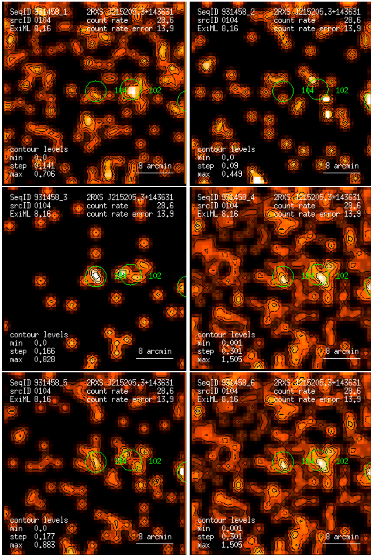
Figure 104: RASS 931458: detection 0104: band rate images, Gaussian filter: (1) PSPC channels 11 – 41, (2) 52 – 90, (3) 91 – 201, (4) 11 – 235, (5) 52 – 201, (6) 11 – 201. Broad band rates in counts/ks. Band rate contour levels in counts/ks/arcmin 2 .
