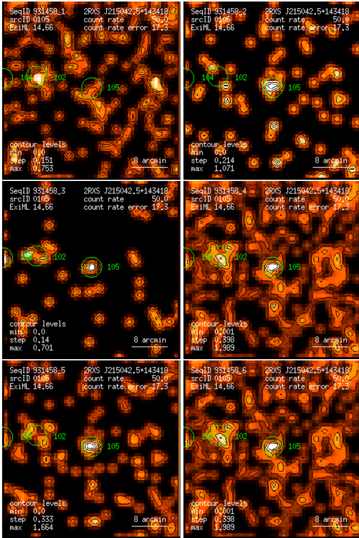
Figure 105: RASS 931458: detection 0105: band rate images, Gaussian filter: (1) PSPC channels 11 – 41, (2) 52 – 90, (3) 91 – 201, (4) 11 – 235, (5) 52 – 201, (6) 11 – 201. Broad band rates in counts/ks. Band rate contour levels in counts/ks/arcmin 2 .
