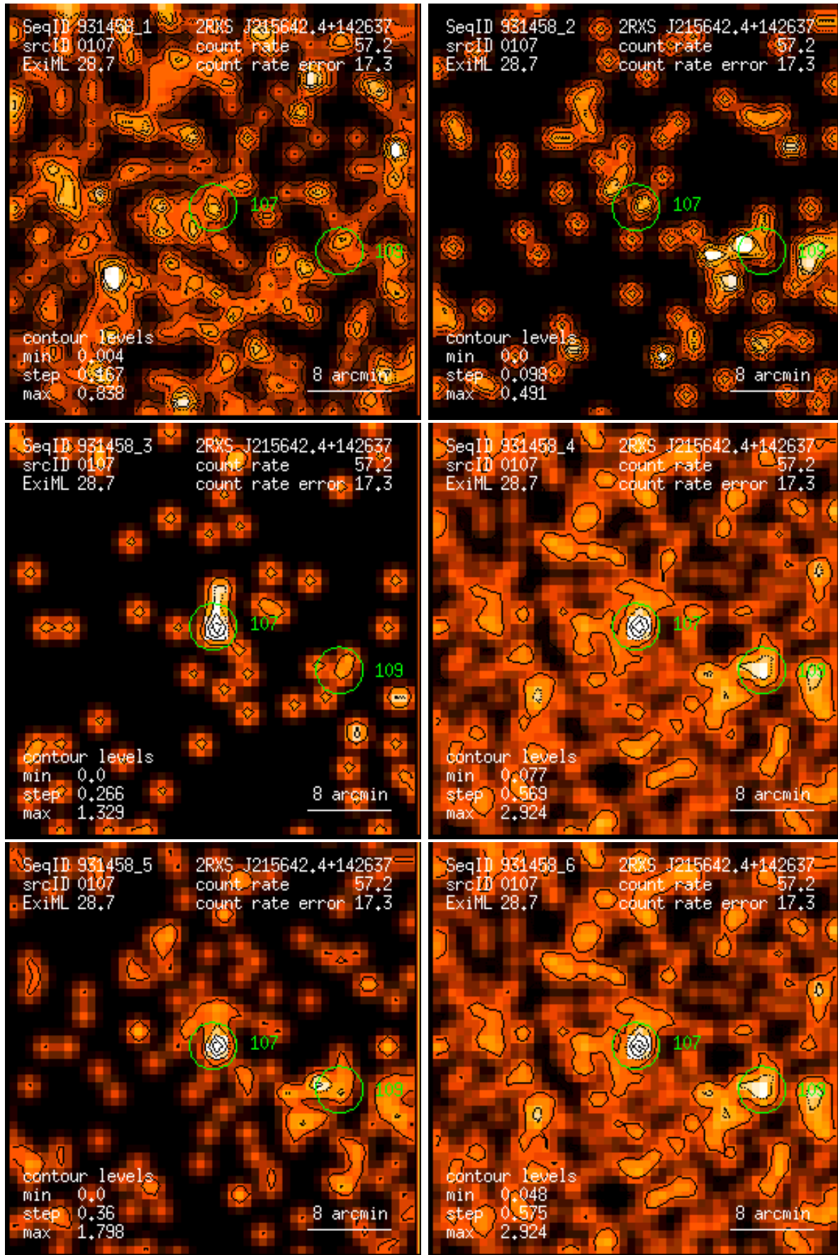
Figure 107: RASS 931458: detection 0107: band rate images, Gaussian filter: (1) PSPC channels 11 – 41, (2) 52 – 90, (3) 91 – 201, (4) 11 – 235, (5) 52 – 201, (6) 11 – 201. Broad band rates in counts/ks. Band rate contour levels in counts/ks/arcmin 2 .
