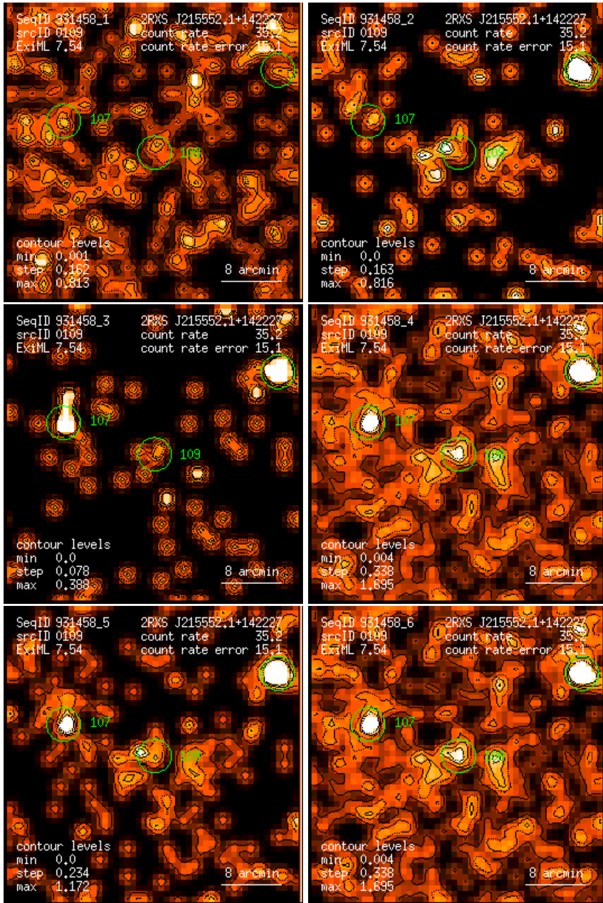
Figure 109: RASS 931458: detection 0109: band rate images, Gaussian filter: (1) PSPC channels 11 – 41, (2) 52 – 90, (3) 91 – 201, (4) 11 – 235, (5) 52 – 201, (6) 11 – 201. Broad band rates in counts/ks. Band rate contour levels in counts/ks/arcmin 2 .
