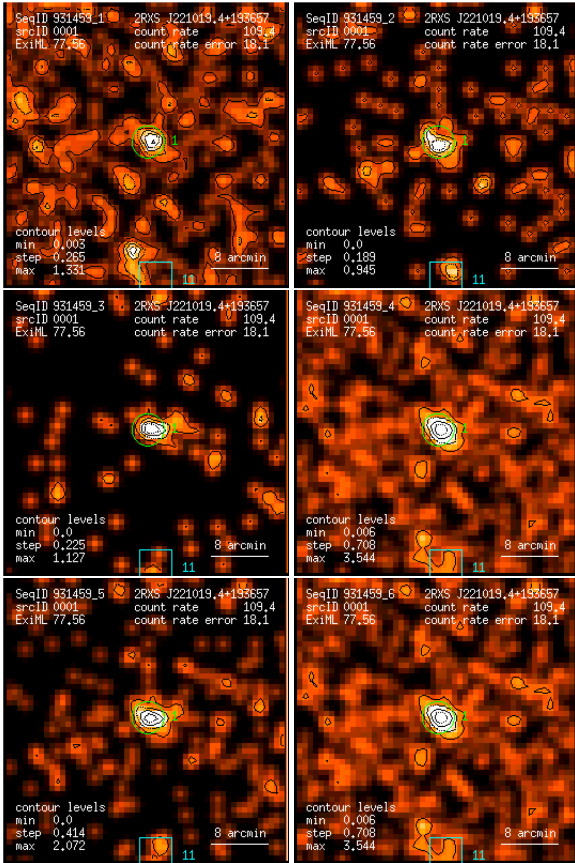
Figure 1: RASS 931459: detection 0001: band rate images, Gaussian filter: (1) PSPC channels 11 – 41, (2) 52 – 90, (3) 91 – 201, (4) 11 – 235, (5) 52 – 201, (6) 11 – 201. Broad band rates in counts/ks. Band rate contour levels in counts/ks/arcmin 2 .
