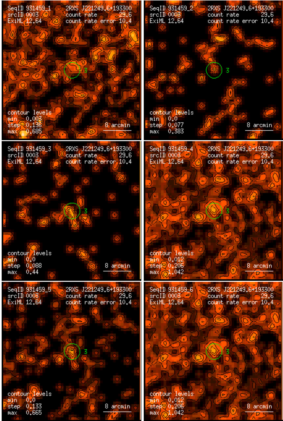
Figure 3: RASS 931459: detection 0003: band rate images, Gaussian filter: (1) PSPC channels 11 – 41, (2) 52 – 90, (3) 91 – 201, (4) 11 – 235, (5) 52 – 201, (6) 11 – 201. Broad band rates in counts/ks. Band rate contour levels in counts/ks/arcmin 2 .
