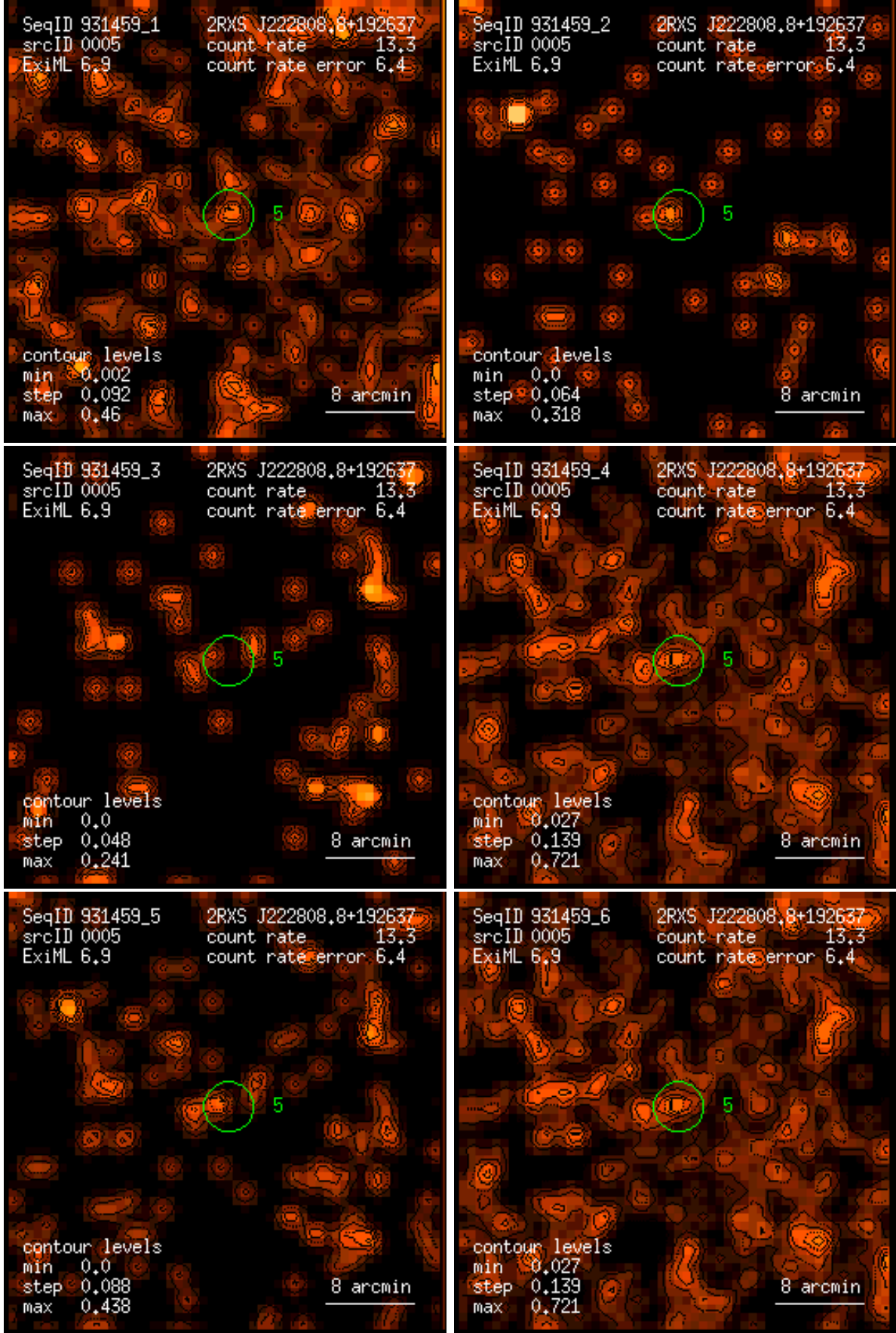
Figure 5: RASS 931459: detection 0005: band rate images, Gaussian filter: (1) PSPC channels 11 – 41, (2) 52 – 90, (3) 91 – 201, (4) 11 – 235, (5) 52 – 201, (6) 11 – 201. Broad band rates in counts/ks. Band rate contour levels in counts/ks/arcmin 2 .
