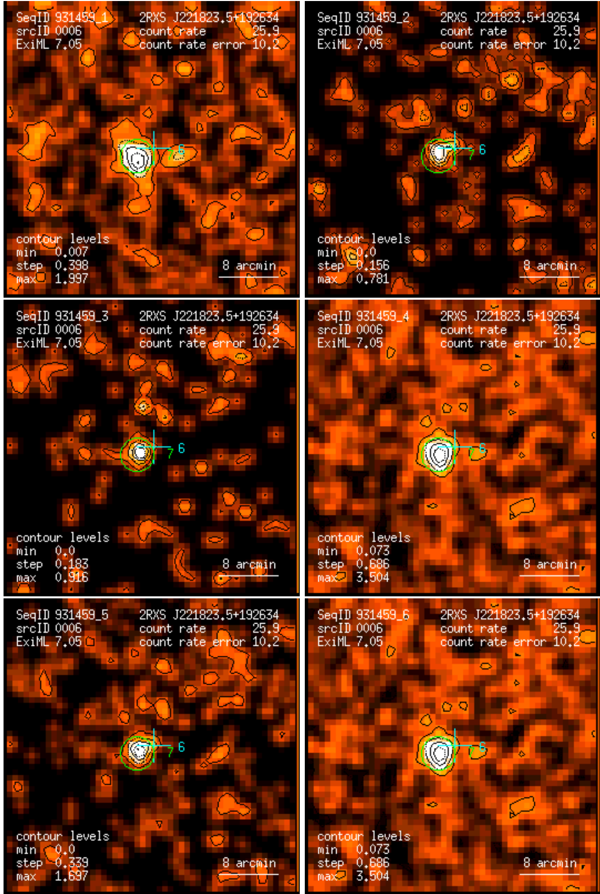
Figure 6: RASS 931459: detection 0006: band rate images, Gaussian filter: (1) PSPC channels 11 – 41, (2) 52 – 90, (3) 91 – 201, (4) 11 – 235, (5) 52 – 201, (6) 11 – 201. Broad band rates in counts/ks. Band rate contour levels in counts/ks/arcmin 2 .
