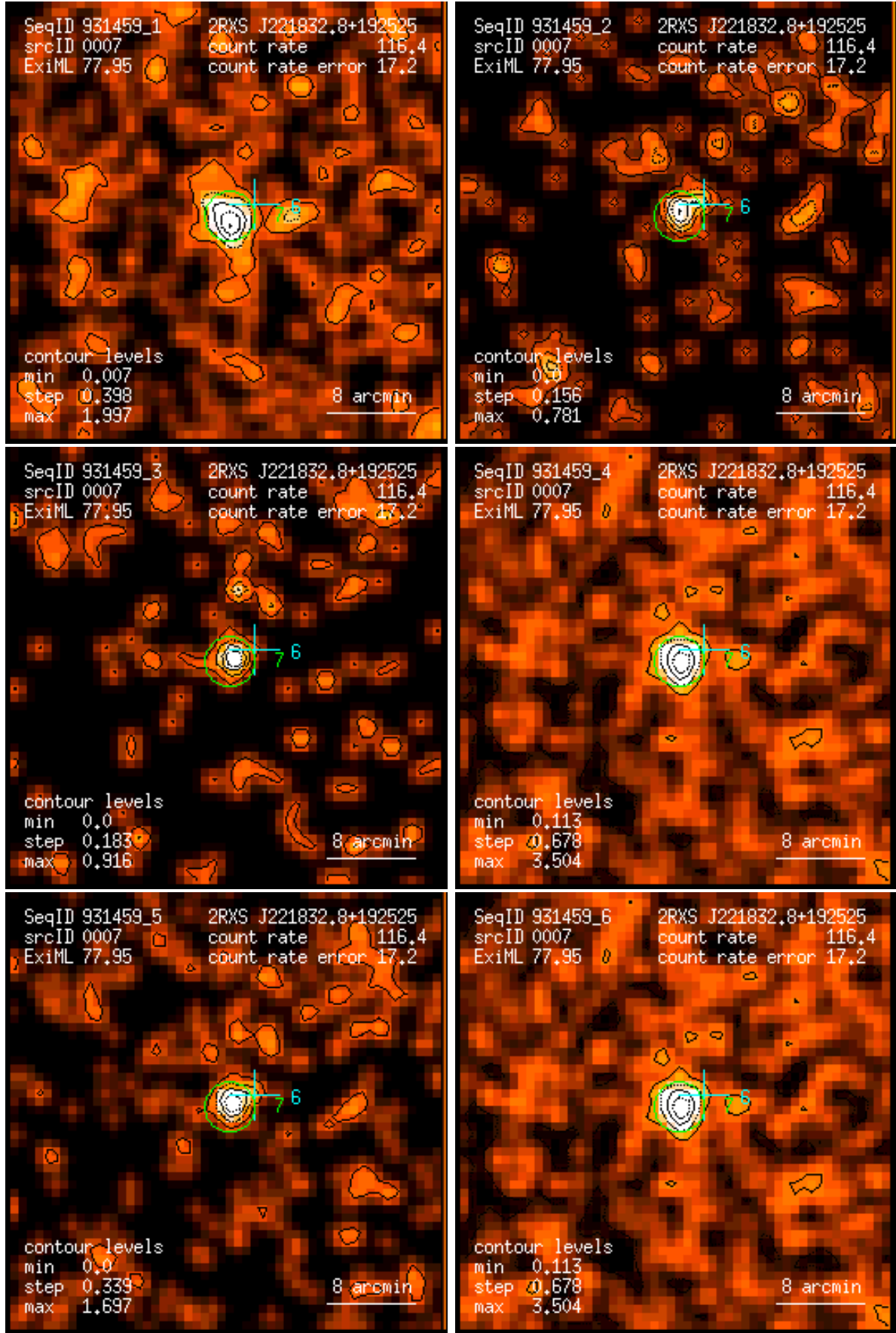
Figure 7: RASS 931459: detection 0007: band rate images, Gaussian filter: (1) PSPC channels 11 – 41, (2) 52 – 90, (3) 91 – 201, (4) 11 – 235, (5) 52 – 201, (6) 11 – 201. Broad band rates in counts/ks. Band rate contour levels in counts/ks/arcmin 2 .
