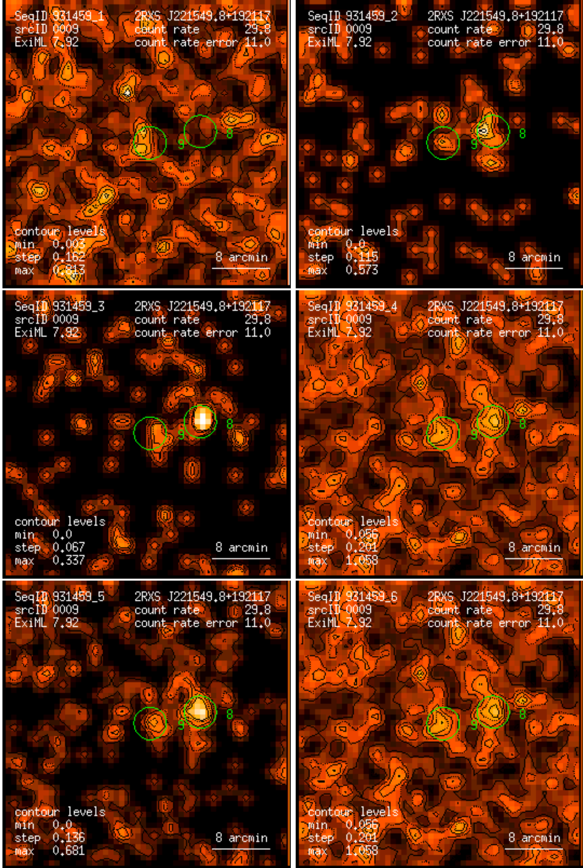
Figure 9: RASS 931459: detection 0009: band rate images, Gaussian filter: (1) PSPC channels 11 – 41, (2) 52 – 90, (3) 91 – 201, (4) 11 – 235, (5) 52 – 201, (6) 11 – 201. Broad band rates in counts/ks. Band rate contour levels in counts/ks/arcmin 2 .
