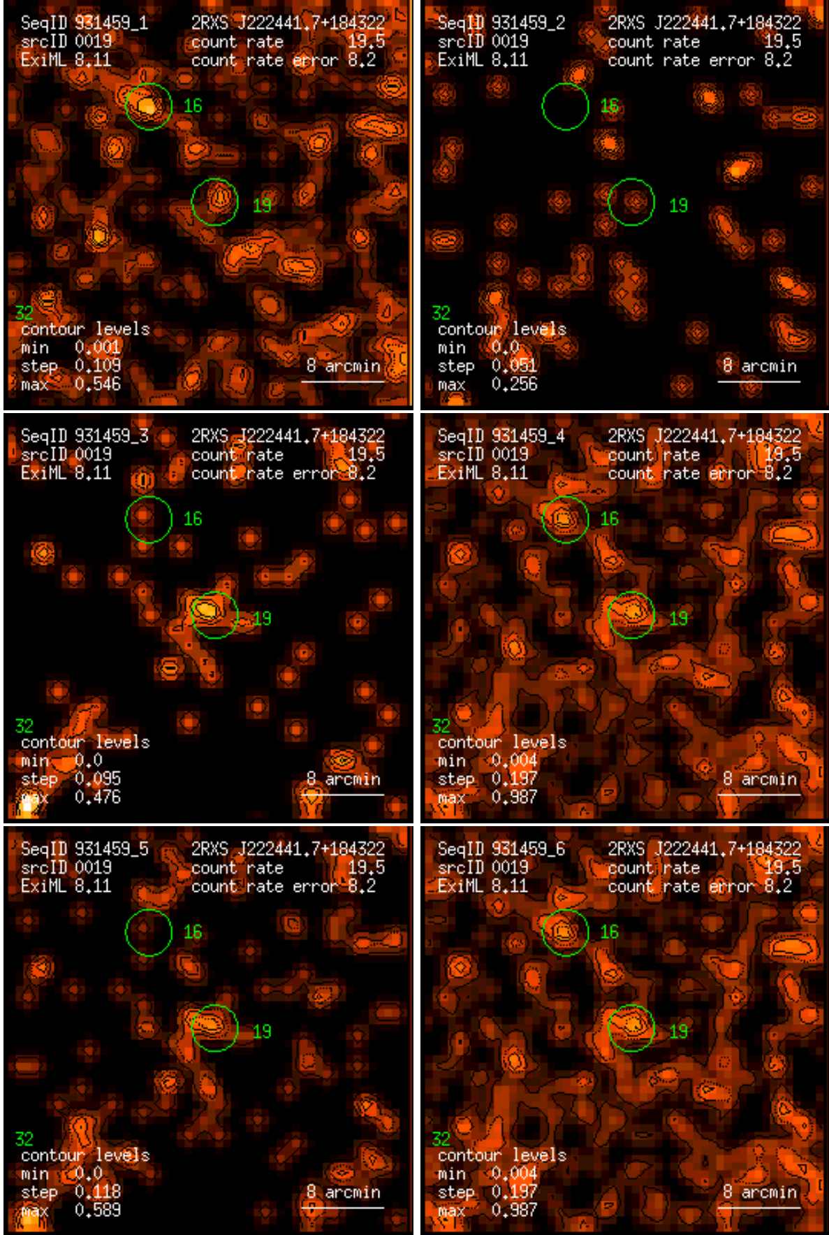
Figure 19: RASS 931459: detection 0019: band rate images, Gaussian filter: (1) PSPC channels 11 – 41, (2) 52 – 90, (3) 91 – 201, (4) 11 – 235, (5) 52 – 201, (6) 11 – 201. Broad band rates in counts/ks. Band rate contour levels in counts/ks/arcmin 2 .
