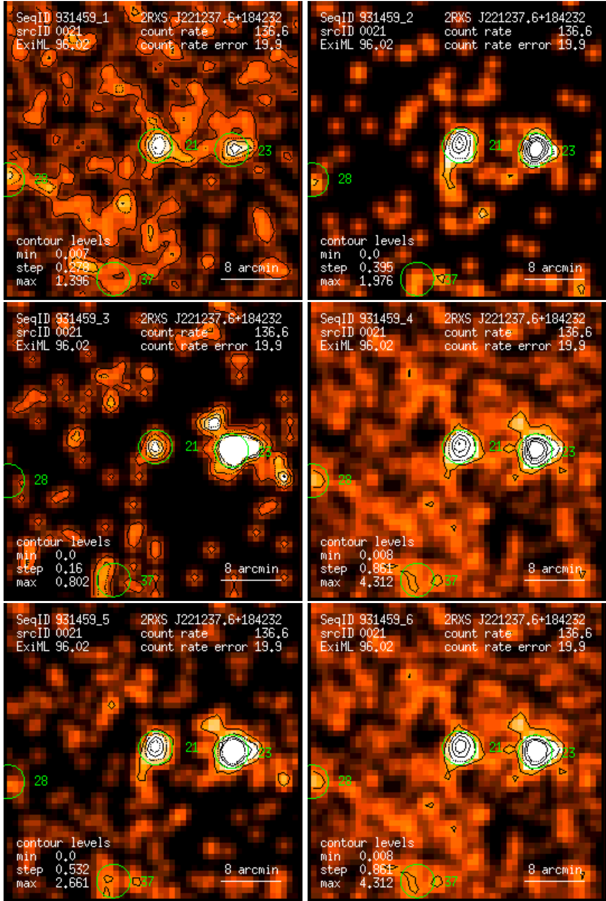
Figure 21: RASS 931459: detection 0021: band rate images, Gaussian filter: (1) PSPC channels 11 – 41, (2) 52 – 90, (3) 91 – 201, (4) 11 – 235, (5) 52 – 201, (6) 11 – 201. Broad band rates in counts/ks. Band rate contour levels in counts/ks/arcmin 2 .
