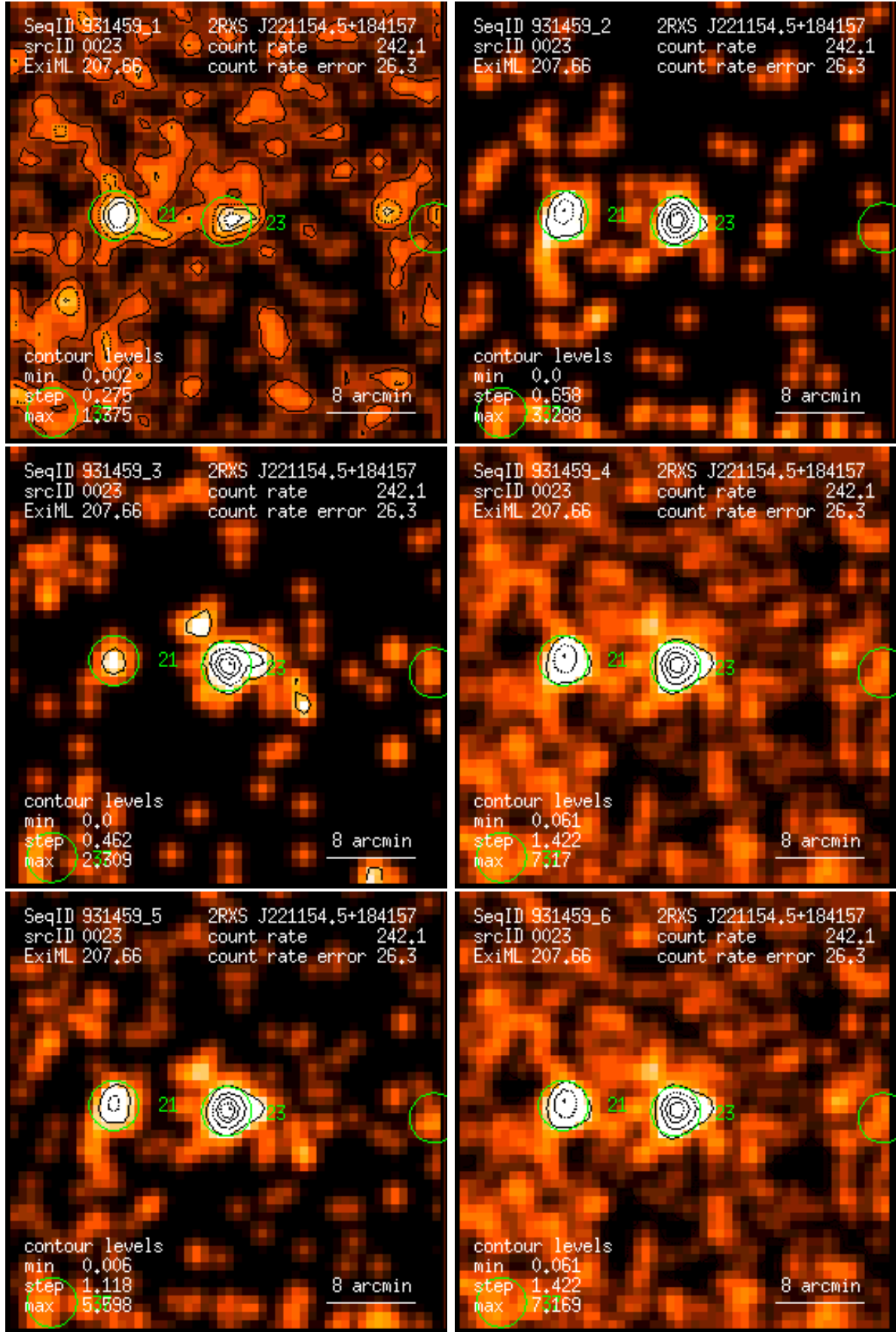
Figure 23: RASS 931459: detection 0023: band rate images, Gaussian filter: (1) PSPC channels 11 – 41, (2) 52 – 90, (3) 91 – 201, (4) 11 – 235, (5) 52 – 201, (6) 11 – 201. Broad band rates in counts/ks. Band rate contour levels in counts/ks/arcmin 2 .
