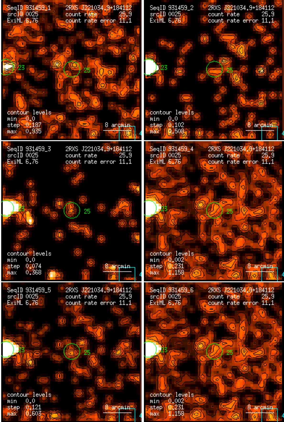
Figure 25: RASS 931459: detection 0025: band rate images, Gaussian filter: (1) PSPC channels 11 – 41, (2) 52 – 90, (3) 91 – 201, (4) 11 – 235, (5) 52 – 201, (6) 11 – 201. Broad band rates in counts/ks. Band rate contour levels in counts/ks/arcmin 2 .
