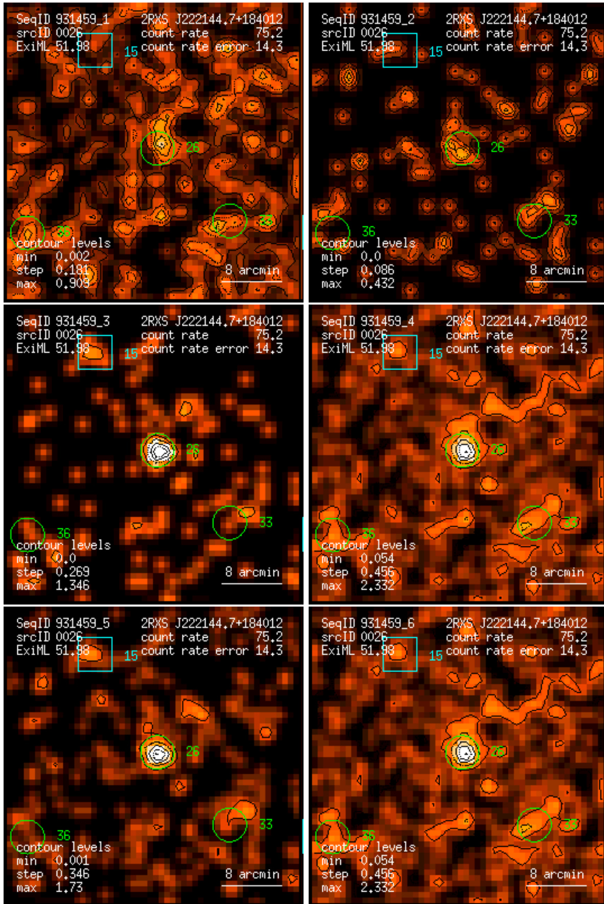
Figure 26: RASS 931459: detection 0026: band rate images, Gaussian filter: (1) PSPC channels 11 – 41, (2) 52 – 90, (3) 91 – 201, (4) 11 – 235, (5) 52 – 201, (6) 11 – 201. Broad band rates in counts/ks. Band rate contour levels in counts/ks/arcmin 2 .
