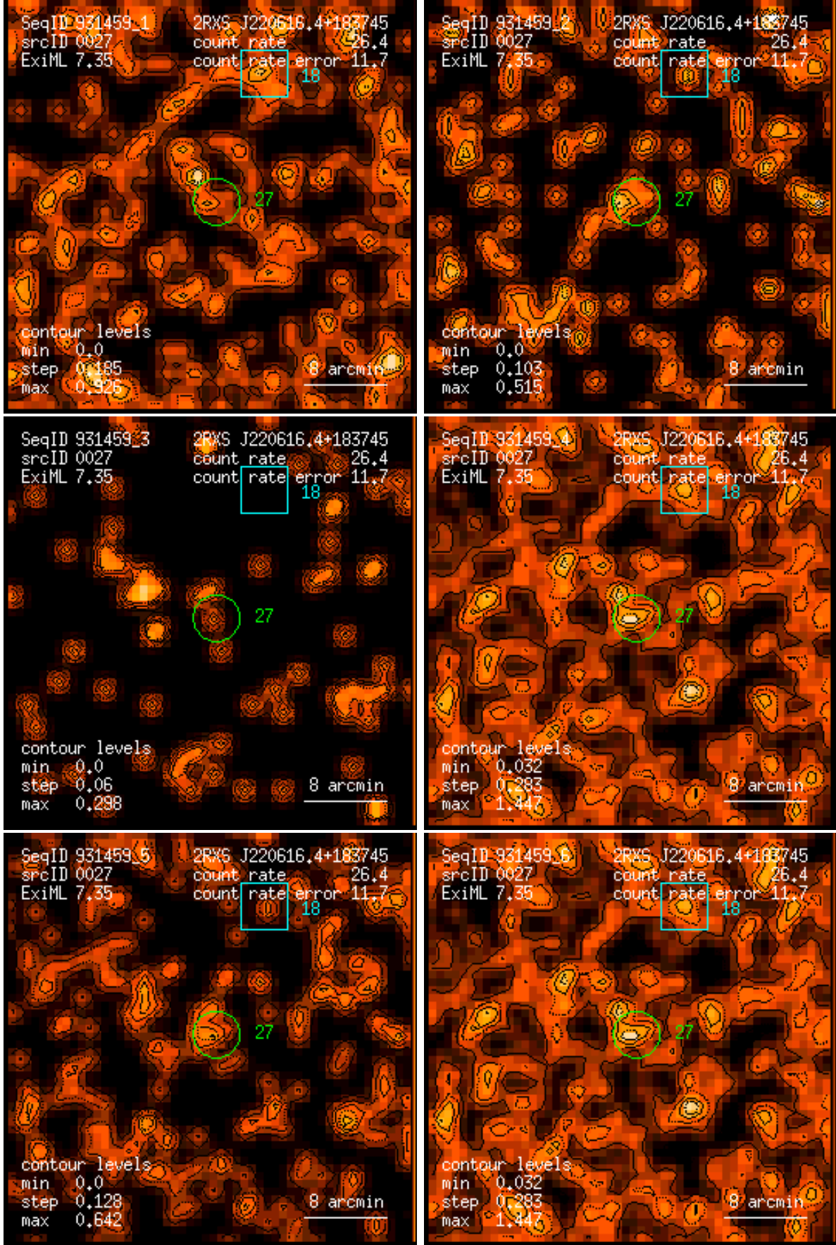
Figure 27: RASS 931459: detection 0027: band rate images, Gaussian filter: (1) PSPC channels 11 – 41, (2) 52 – 90, (3) 91 – 201, (4) 11 – 235, (5) 52 – 201, (6) 11 – 201. Broad band rates in counts/ks. Band rate contour levels in counts/ks/arcmin 2 .
