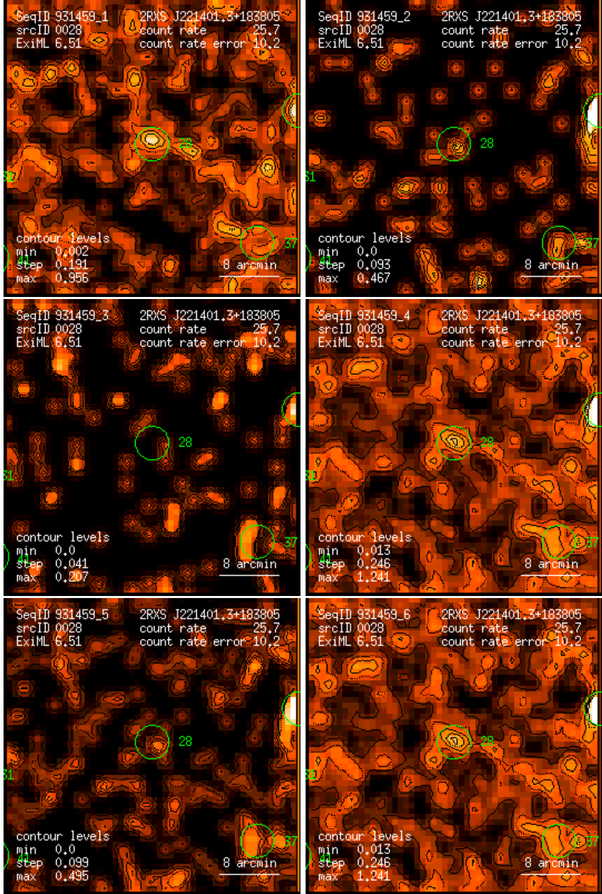
Figure 28: RASS 931459: detection 0028: band rate images, Gaussian filter: (1) PSPC channels 11 – 41, (2) 52 – 90, (3) 91 – 201, (4) 11 – 235, (5) 52 – 201, (6) 11 – 201. Broad band rates in counts/ks. Band rate contour levels in counts/ks/arcmin 2 .
