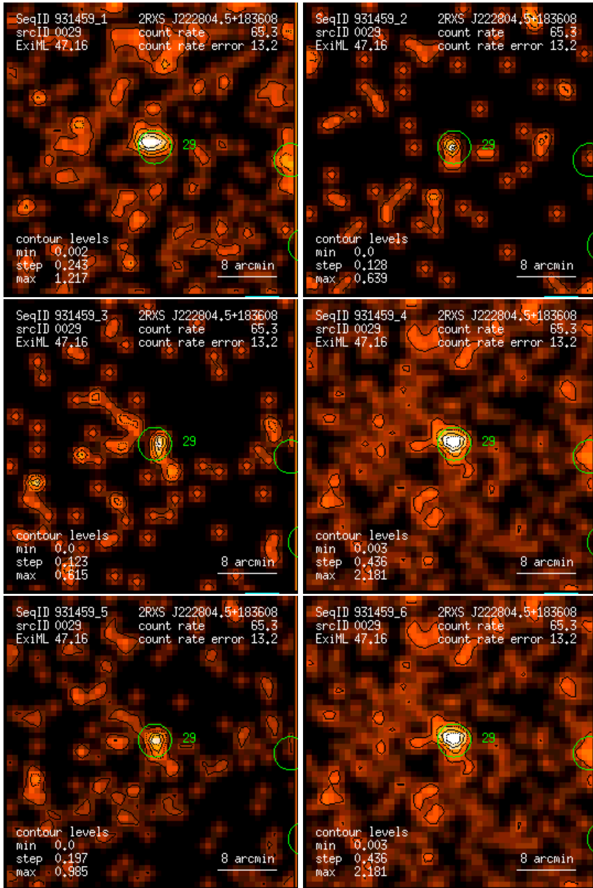
Figure 29: RASS 931459: detection 0029: band rate images, Gaussian filter: (1) PSPC channels 11 – 41, (2) 52 – 90, (3) 91 – 201, (4) 11 – 235, (5) 52 – 201, (6) 11 – 201. Broad band rates in counts/ks. Band rate contour levels in counts/ks/arcmin 2 .
