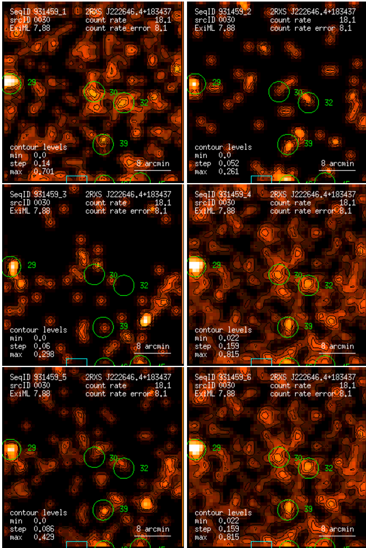
Figure 30: RASS 931459: detection 0030: band rate images, Gaussian filter: (1) PSPC channels 11 – 41, (2) 52 – 90, (3) 91 – 201, (4) 11 – 235, (5) 52 – 201, (6) 11 – 201. Broad band rates in counts/ks. Band rate contour levels in counts/ks/arcmin 2 .
