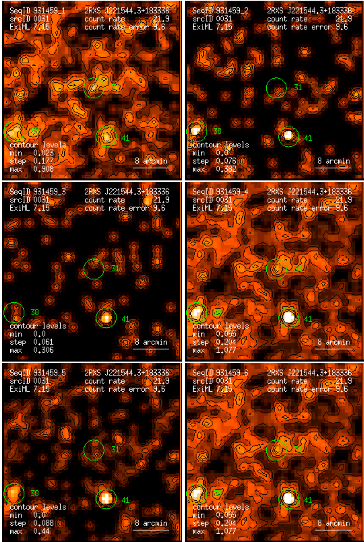
Figure 31: RASS 931459: detection 0031: band rate images, Gaussian filter: (1) PSPC channels 11 – 41, (2) 52 – 90, (3) 91 – 201, (4) 11 – 235, (5) 52 – 201, (6) 11 – 201. Broad band rates in counts/ks. Band rate contour levels in counts/ks/arcmin 2 .
