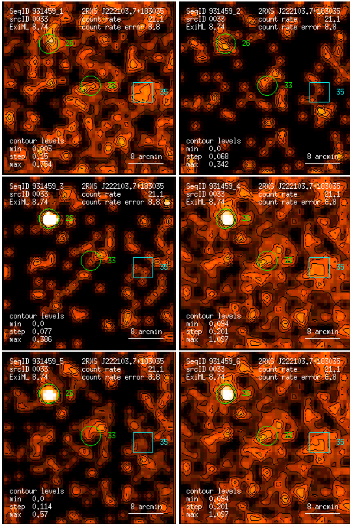
Figure 33: RASS 931459: detection 0033: band rate images, Gaussian filter: (1) PSPC channels 11 – 41, (2) 52 – 90, (3) 91 – 201, (4) 11 – 235, (5) 52 – 201, (6) 11 – 201. Broad band rates in counts/ks. Band rate contour levels in counts/ks/arcmin 2 .
