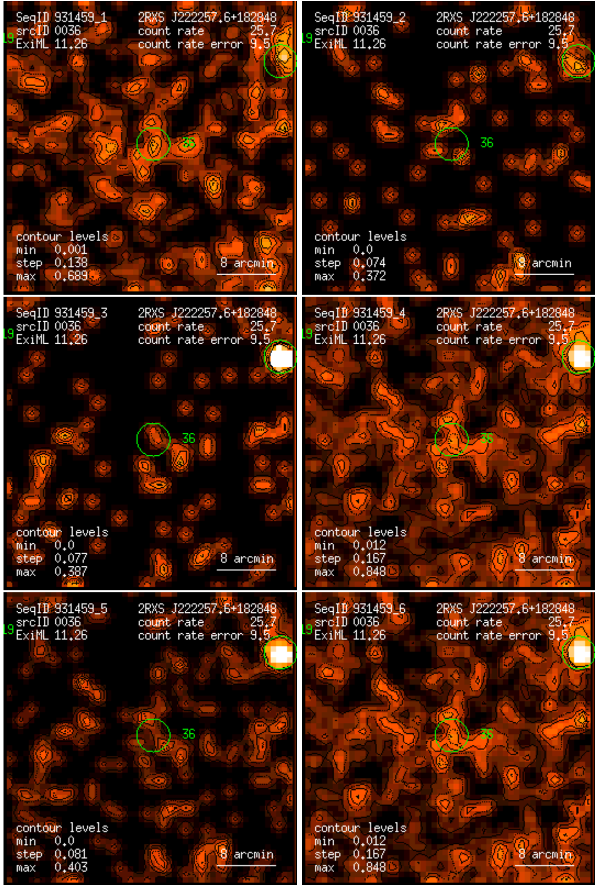
Figure 36: RASS 931459: detection 0036: band rate images, Gaussian filter: (1) PSPC channels 11 – 41, (2) 52 – 90, (3) 91 – 201, (4) 11 – 235, (5) 52 – 201, (6) 11 – 201. Broad band rates in counts/ks. Band rate contour levels in counts/ks/arcmin 2 .
