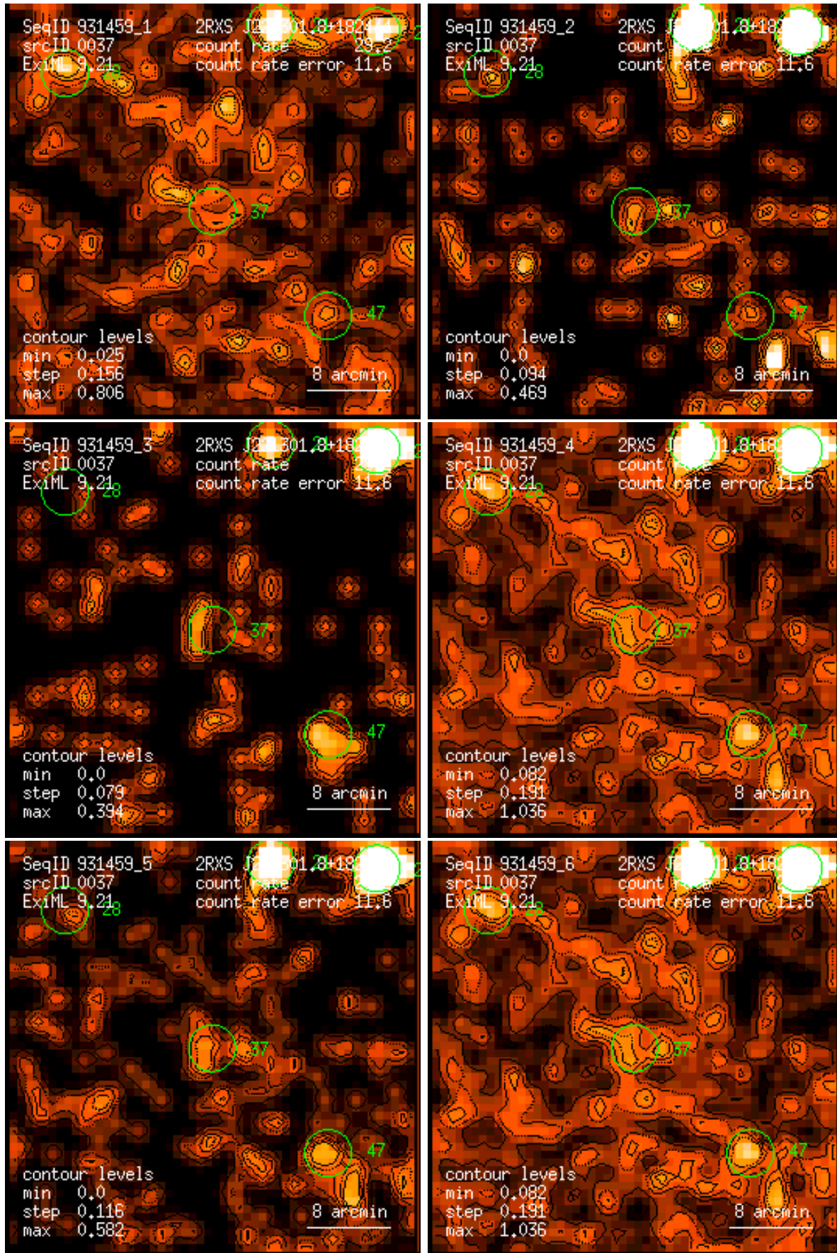
Figure 37: RASS 931459: detection 0037: band rate images, Gaussian filter: (1) PSPC channels 11 – 41, (2) 52 – 90, (3) 91 – 201, (4) 11 – 235, (5) 52 – 201, (6) 11 – 201. Broad band rates in counts/ks. Band rate contour levels in counts/ks/arcmin 2 .
