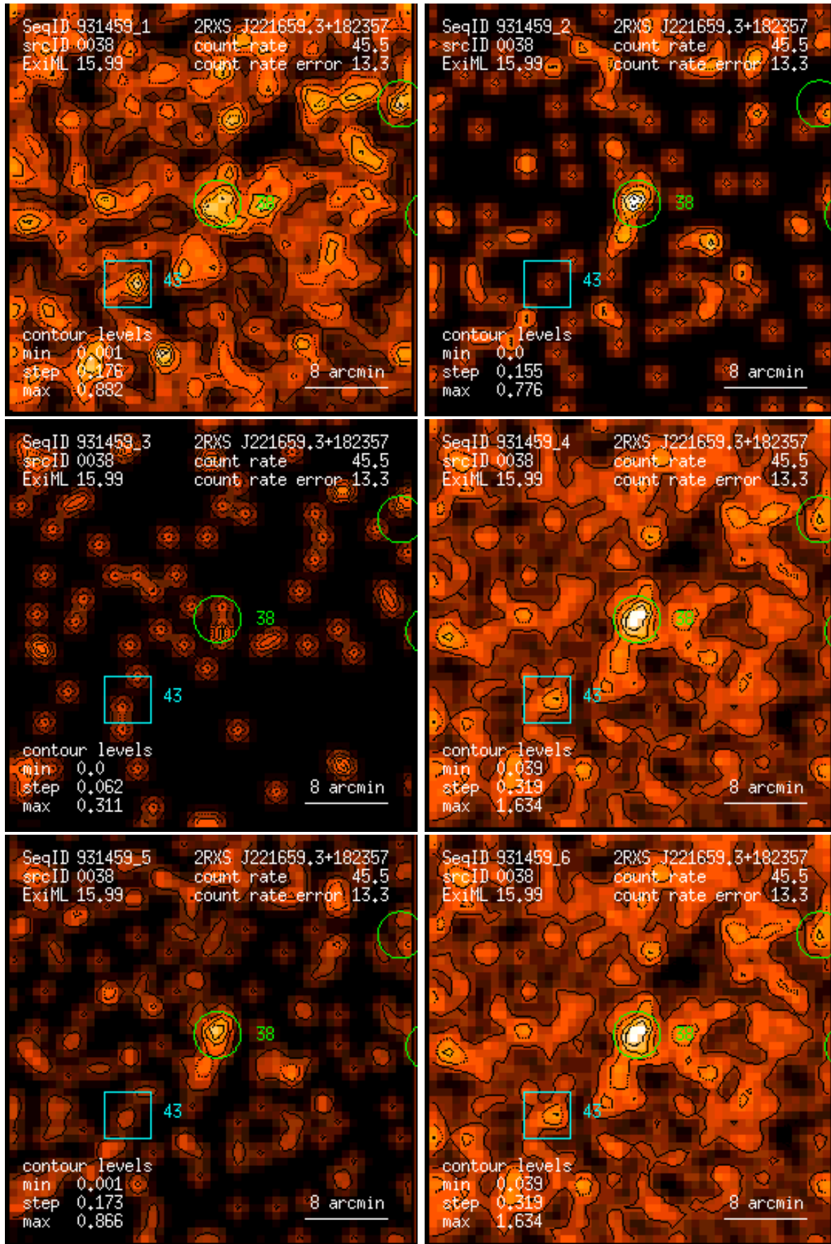
Figure 38: RASS 931459: detection 0038: band rate images, Gaussian filter: (1) PSPC channels 11 – 41, (2) 52 – 90, (3) 91 – 201, (4) 11 – 235, (5) 52 – 201, (6) 11 – 201. Broad band rates in counts/ks. Band rate contour levels in counts/ks/arcmin 2 .
