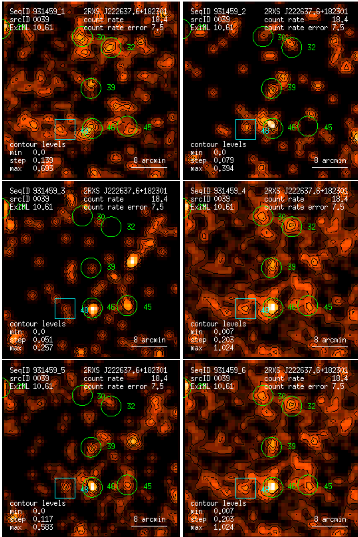
Figure 39: RASS 931459: detection 0039: band rate images, Gaussian filter: (1) PSPC channels 11 – 41, (2) 52 – 90, (3) 91 – 201, (4) 11 – 235, (5) 52 – 201, (6) 11 – 201. Broad band rates in counts/ks. Band rate contour levels in counts/ks/arcmin 2 .
