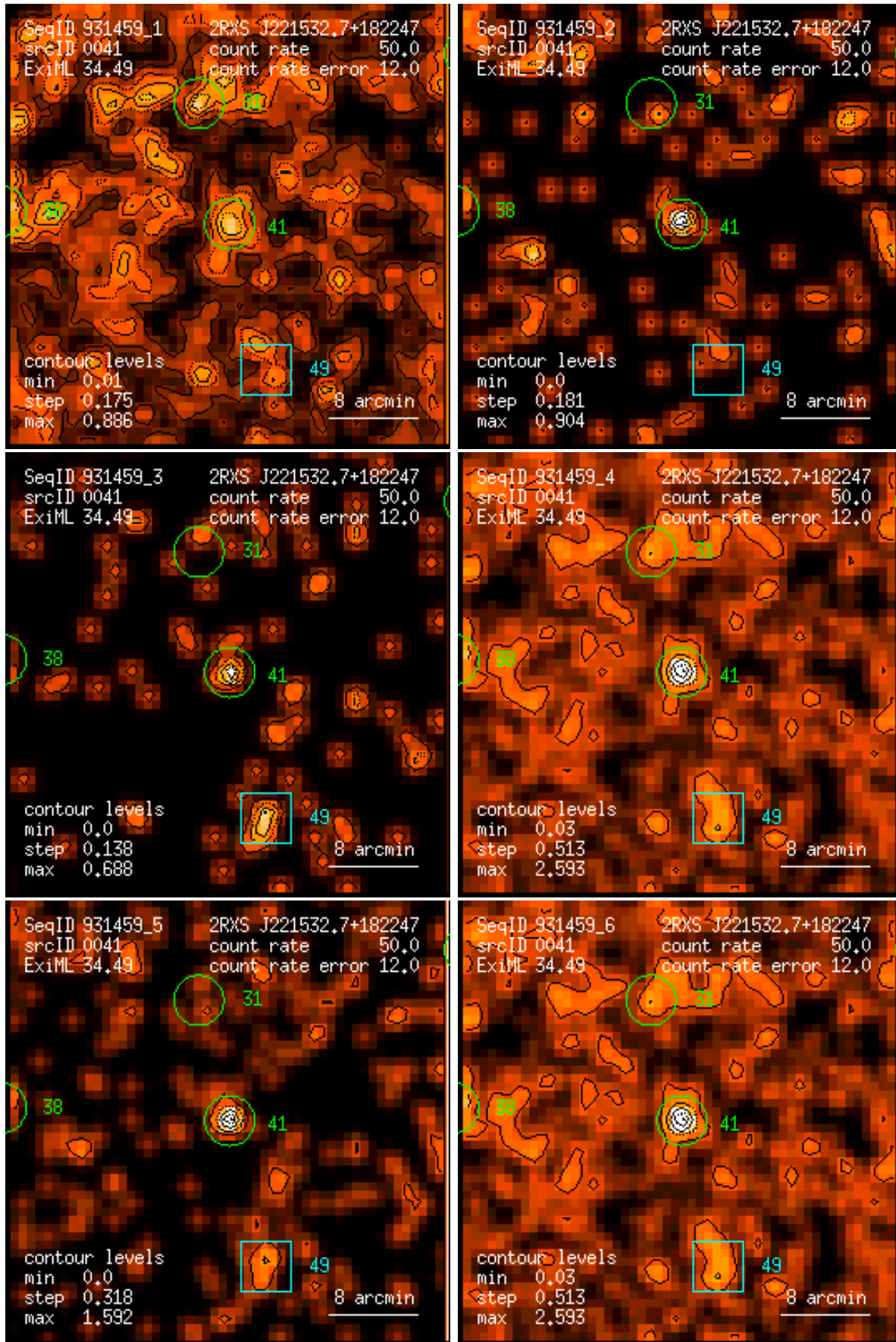
Figure 41: RASS 931459: detection 0041: band rate images, Gaussian filter: (1) PSPC channels 11 – 41, (2) 52 – 90, (3) 91 – 201, (4) 11 – 235, (5) 52 – 201, (6) 11 – 201. Broad band rates in counts/ks. Band rate contour levels in counts/ks/arcmin 2 .
