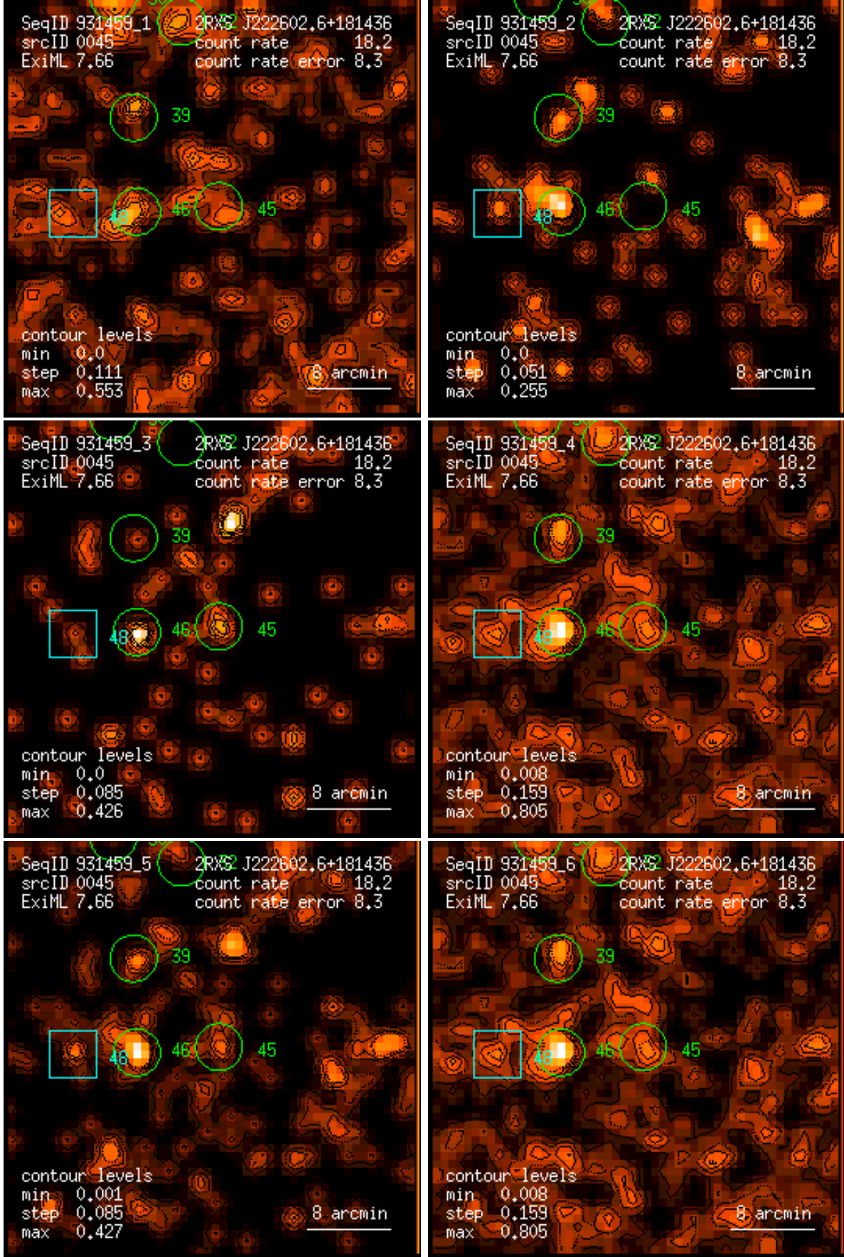
Figure 45: RASS 931459: detection 0045: band rate images, Gaussian filter: (1) PSPC channels 11 – 41, (2) 52 – 90, (3) 91 – 201, (4) 11 – 235, (5) 52 – 201, (6) 11 – 201. Broad band rates in counts/ks. Band rate contour levels in counts/ks/arcmin 2 .
