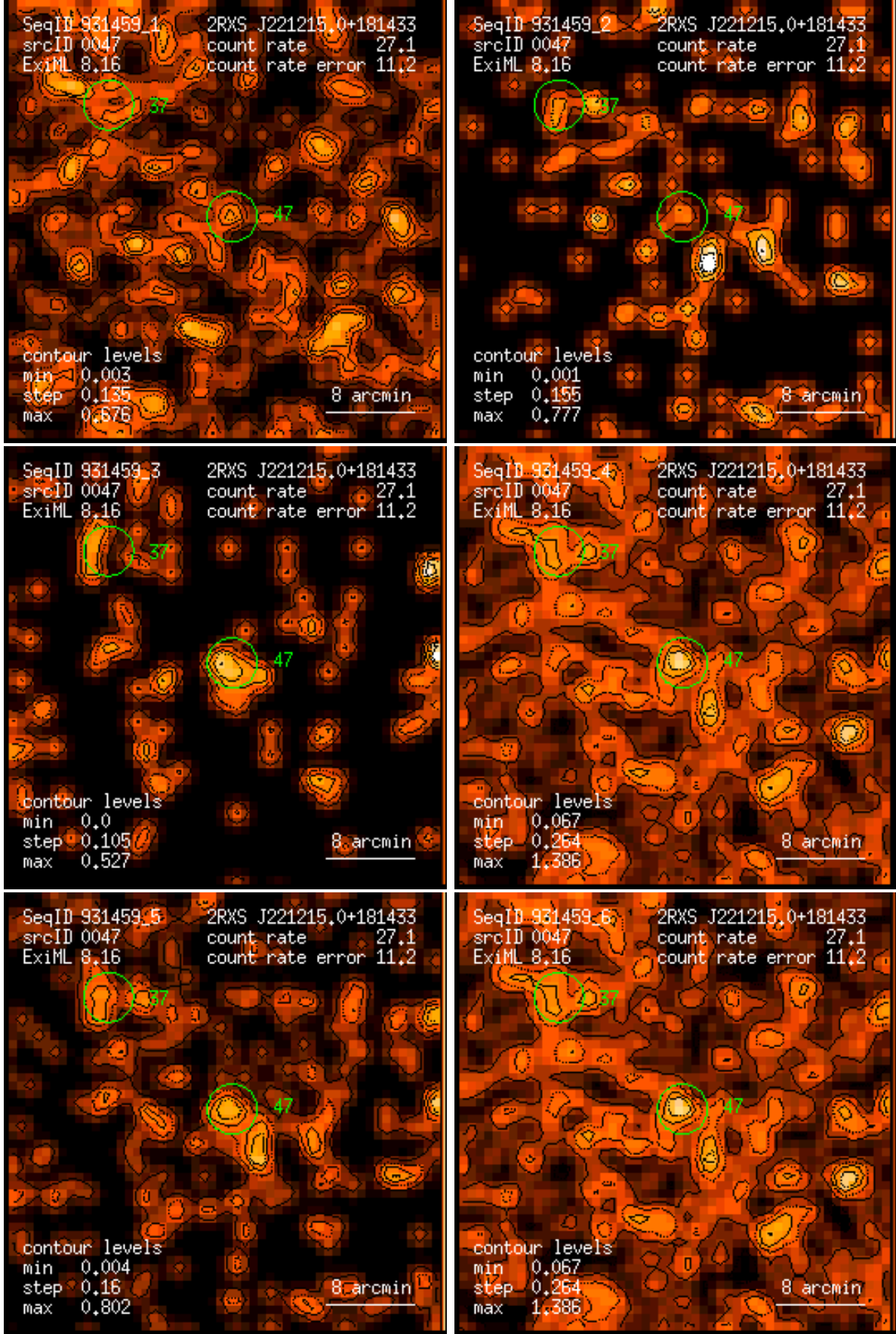
Figure 47: RASS 931459: detection 0047: band rate images, Gaussian filter: (1) PSPC channels 11 – 41, (2) 52 – 90, (3) 91 – 201, (4) 11 – 235, (5) 52 – 201, (6) 11 – 201. Broad band rates in counts/ks. Band rate contour levels in counts/ks/arcmin 2 .
