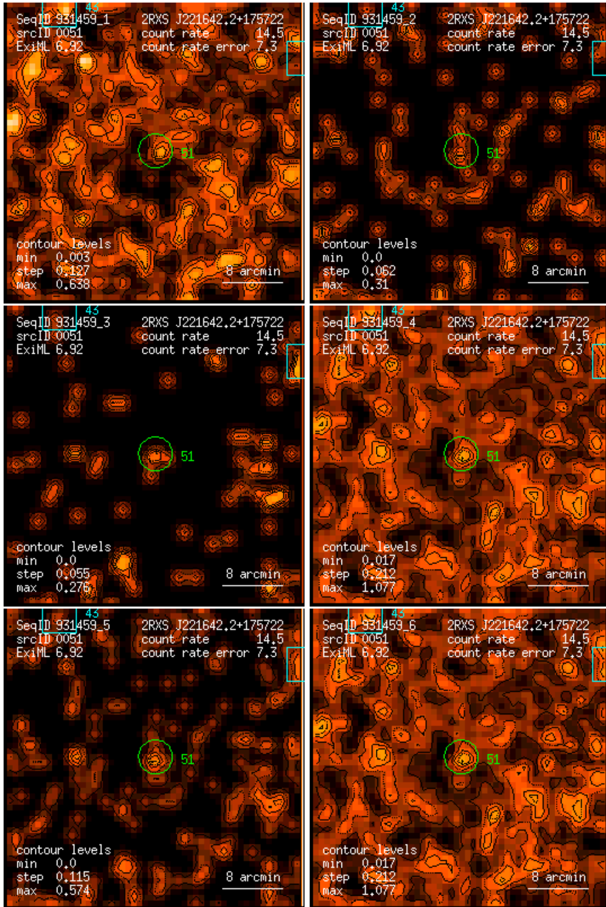
Figure 51: RASS 931459: detection 0051: band rate images, Gaussian filter: (1) PSPC channels 11 – 41, (2) 52 – 90, (3) 91 – 201, (4) 11 – 235, (5) 52 – 201, (6) 11 – 201. Broad band rates in counts/ks. Band rate contour levels in counts/ks/arcmin 2 .
