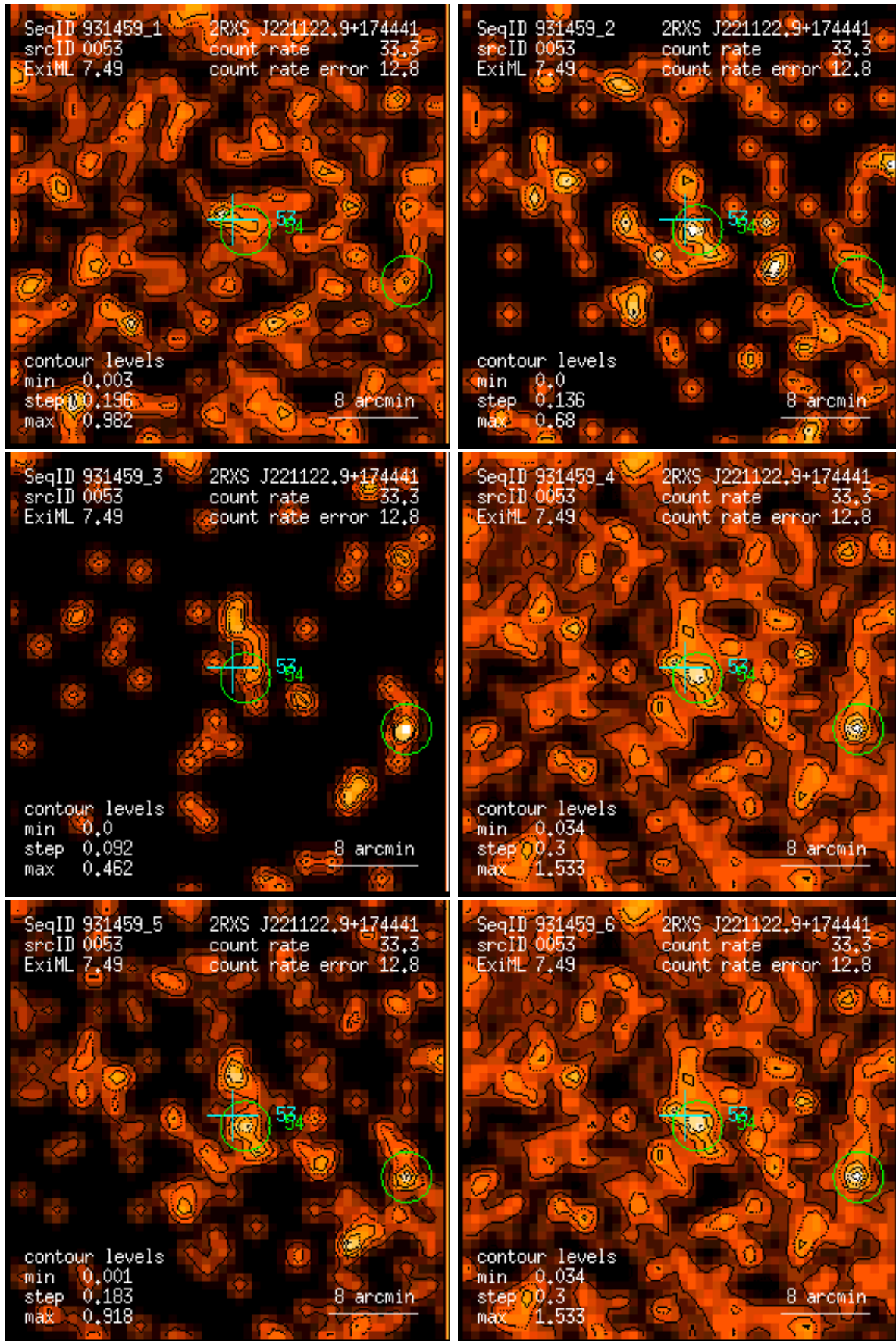
Figure 53: RASS 931459: detection 0053: band rate images, Gaussian filter: (1) PSPC channels 11 – 41, (2) 52 – 90, (3) 91 – 201, (4) 11 – 235, (5) 52 – 201, (6) 11 – 201. Broad band rates in counts/ks. Band rate contour levels in counts/ks/arcmin 2 .
