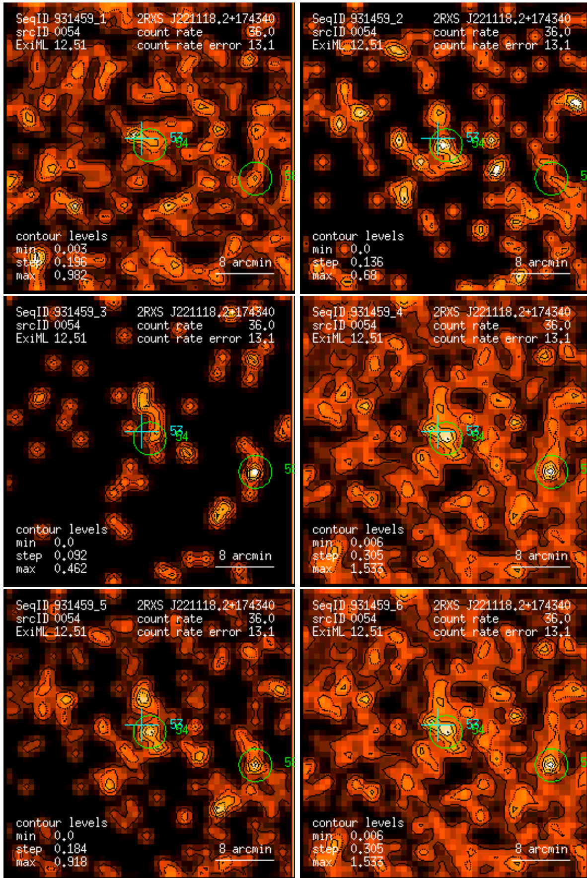
Figure 54: RASS 931459: detection 0054: band rate images, Gaussian filter: (1) PSPC channels 11 – 41, (2) 52 – 90, (3) 91 – 201, (4) 11 – 235, (5) 52 – 201, (6) 11 – 201. Broad band rates in counts/ks. Band rate contour levels in counts/ks/arcmin 2 .
