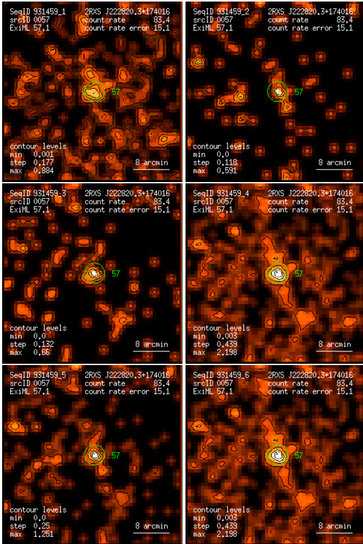
Figure 57: RASS 931459: detection 0057: band rate images, Gaussian filter: (1) PSPC channels 11 – 41, (2) 52 – 90, (3) 91 – 201, (4) 11 – 235, (5) 52 – 201, (6) 11 – 201. Broad band rates in counts/ks. Band rate contour levels in counts/ks/arcmin 2 .
