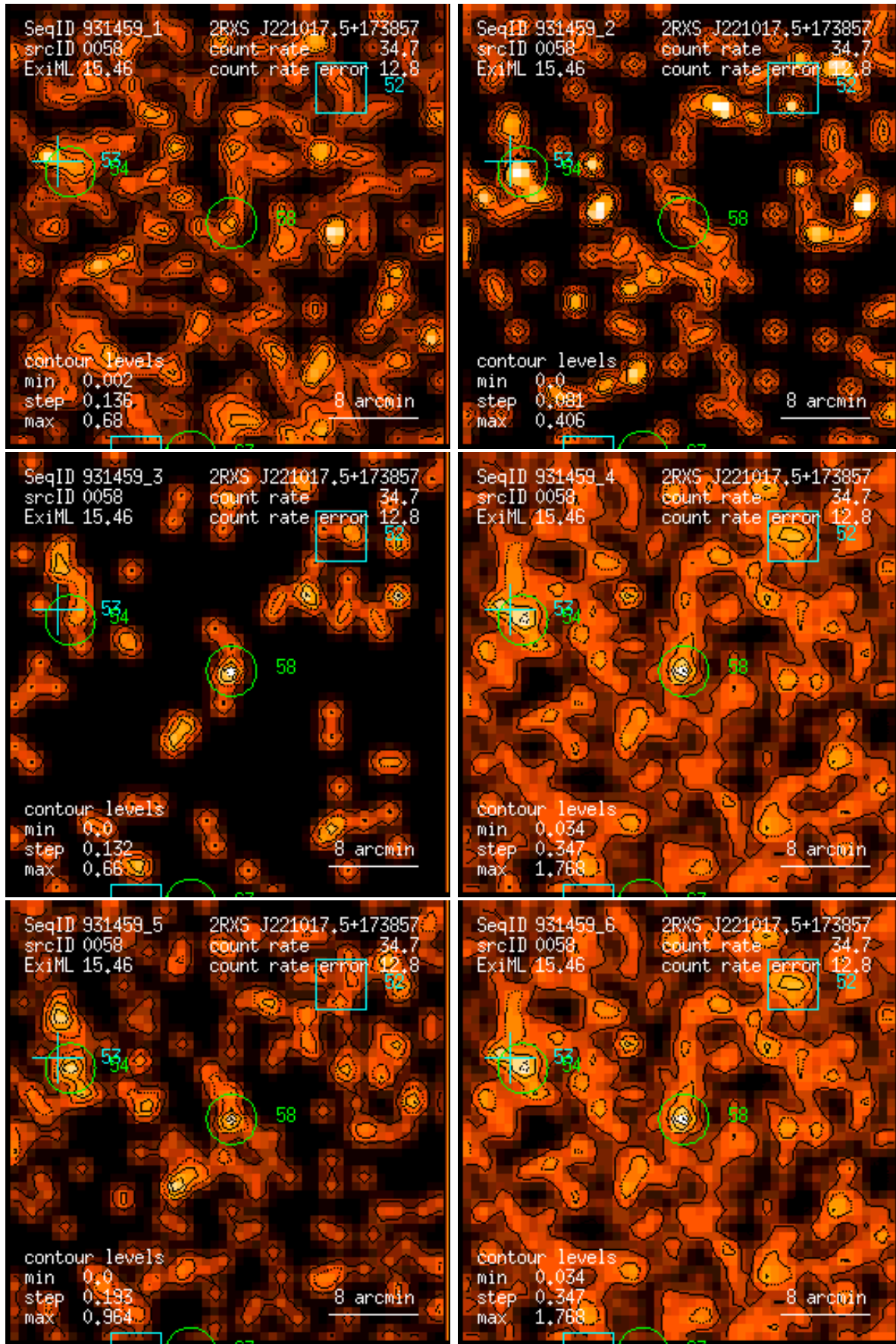
Figure 58: RASS 931459: detection 0058: band rate images, Gaussian filter: (1) PSPC channels 11 – 41, (2) 52 – 90, (3) 91 – 201, (4) 11 – 235, (5) 52 – 201, (6) 11 – 201. Broad band rates in counts/ks. Band rate contour levels in counts/ks/arcmin 2 .
