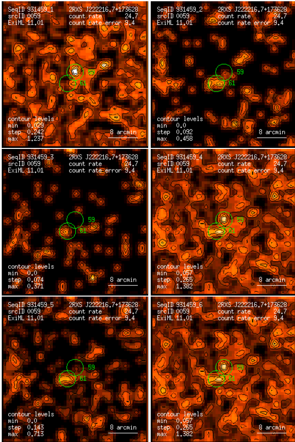
Figure 59: RASS 931459: detection 0059: band rate images, Gaussian filter: (1) PSPC channels 11 – 41, (2) 52 – 90, (3) 91 – 201, (4) 11 – 235, (5) 52 – 201, (6) 11 – 201. Broad band rates in counts/ks. Band rate contour levels in counts/ks/arcmin 2 .
