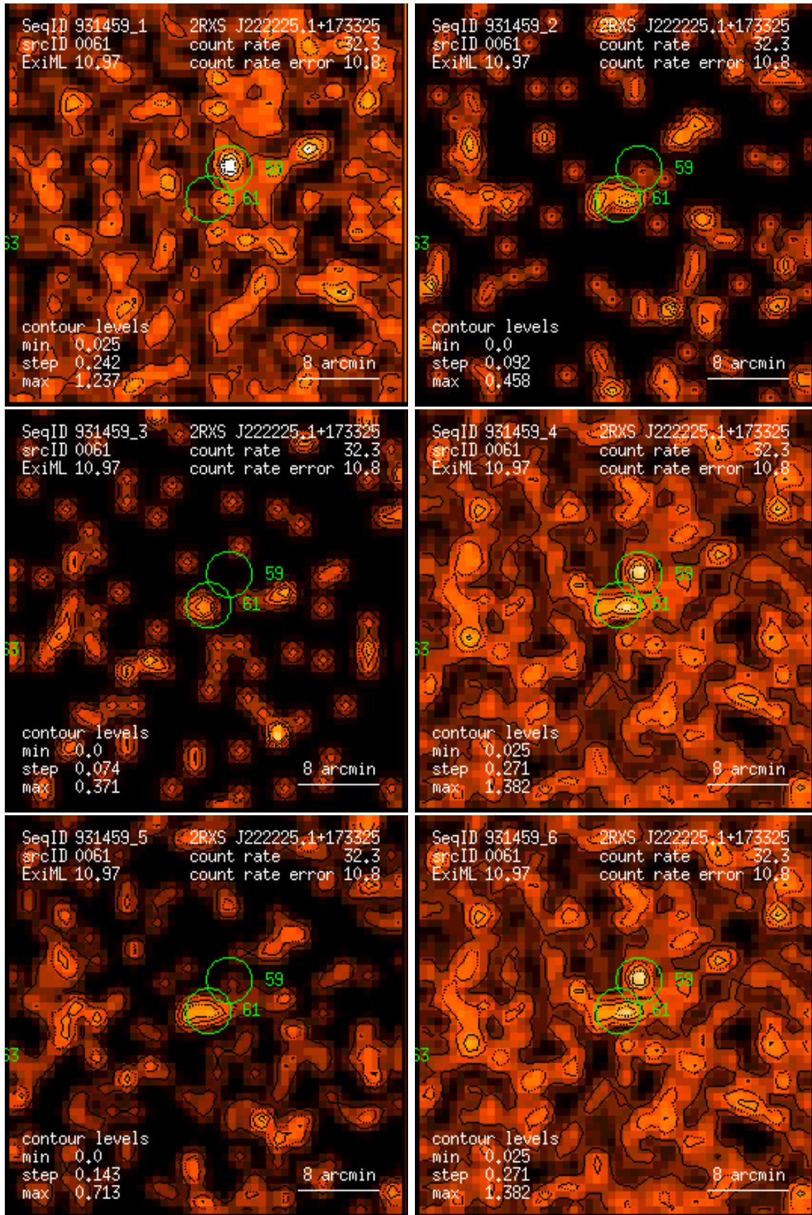
Figure 61: RASS 931459: detection 0061: band rate images, Gaussian filter: (1) PSPC channels 11 – 41, (2) 52 – 90, (3) 91 – 201, (4) 11 – 235, (5) 52 – 201, (6) 11 – 201. Broad band rates in counts/ks. Band rate contour levels in counts/ks/arcmin 2 .
