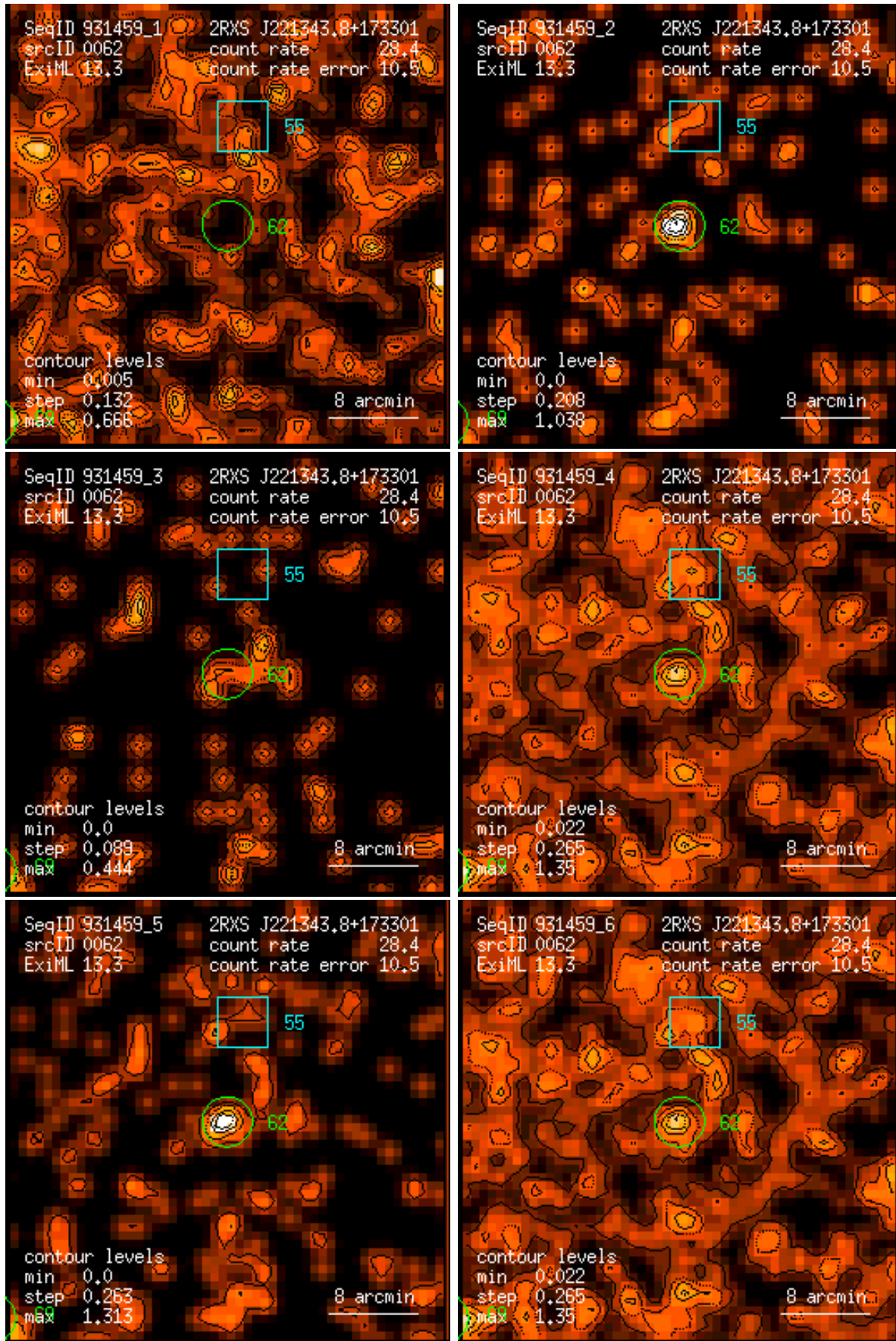
Figure 62: RASS 931459: detection 0062: band rate images, Gaussian filter: (1) PSPC channels 11 – 41, (2) 52 – 90, (3) 91 – 201, (4) 11 – 235, (5) 52 – 201, (6) 11 – 201. Broad band rates in counts/ks. Band rate contour levels in counts/ks/arcmin 2 .
