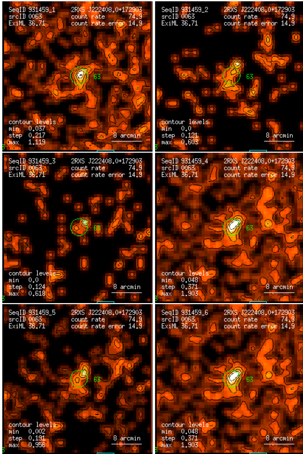
Figure 63: RASS 931459: detection 0063: band rate images, Gaussian filter: (1) PSPC channels 11 – 41, (2) 52 – 90, (3) 91 – 201, (4) 11 – 235, (5) 52 – 201, (6) 11 – 201. Broad band rates in counts/ks. Band rate contour levels in counts/ks/arcmin 2 .
