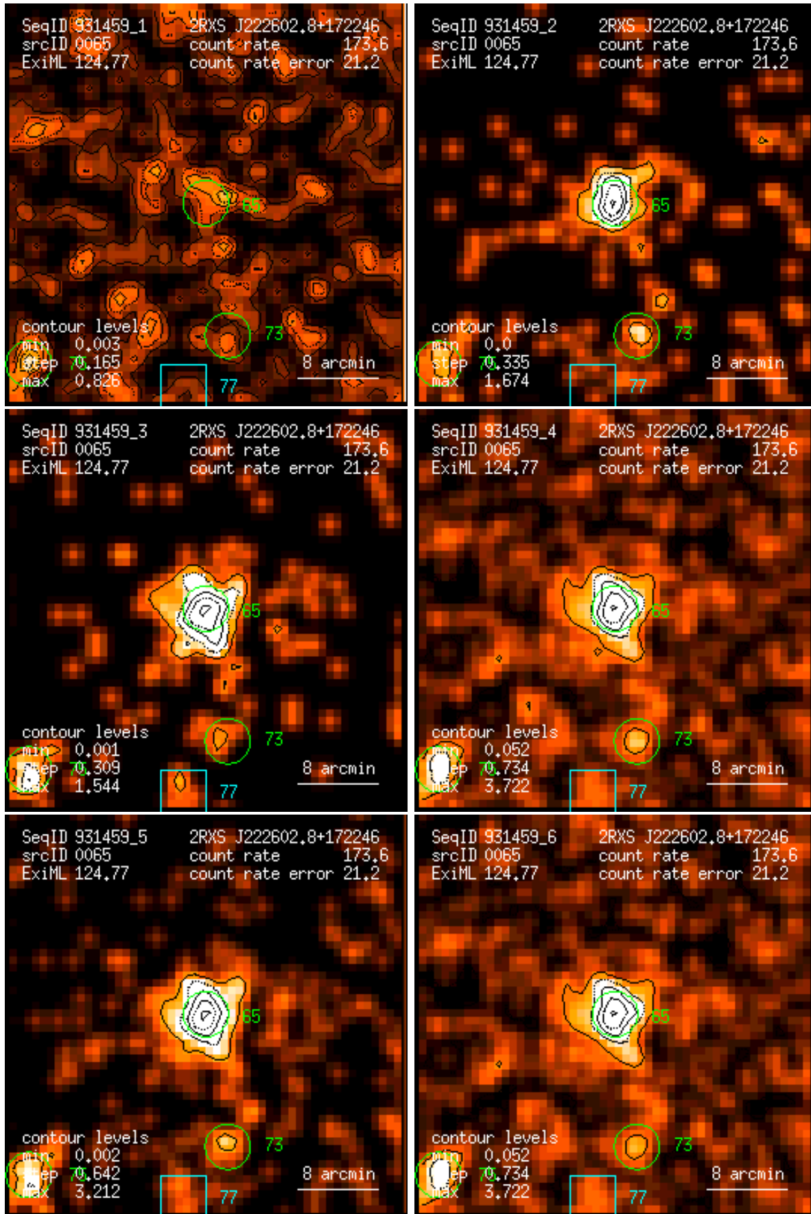
Figure 65: RASS 931459: detection 0065: band rate images, Gaussian filter: (1) PSPC channels 11 – 41, (2) 52 – 90, (3) 91 – 201, (4) 11 – 235, (5) 52 – 201, (6) 11 – 201. Broad band rates in counts/ks. Band rate contour levels in counts/ks/arcmin 2 .
