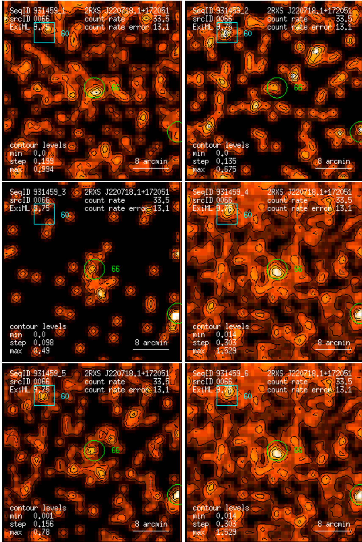
Figure 66: RASS 931459: detection 0066: band rate images, Gaussian filter: (1) PSPC channels 11 – 41, (2) 52 – 90, (3) 91 – 201, (4) 11 – 235, (5) 52 – 201, (6) 11 – 201. Broad band rates in counts/ks. Band rate contour levels in counts/ks/arcmin 2 .
