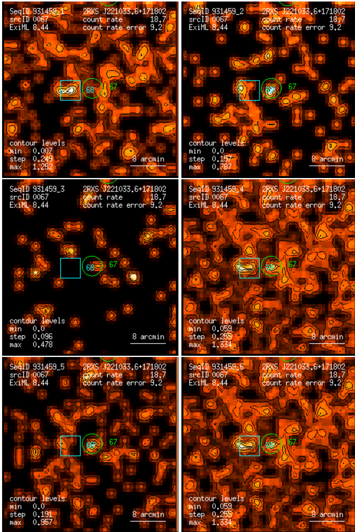
Figure 67: RASS 931459: detection 0067: band rate images, Gaussian filter: (1) PSPC channels 11 – 41, (2) 52 – 90, (3) 91 – 201, (4) 11 – 235, (5) 52 – 201, (6) 11 – 201. Broad band rates in counts/ks. Band rate contour levels in counts/ks/arcmin 2 .
