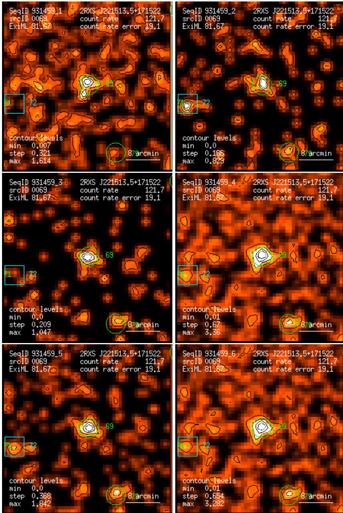
Figure 69: RASS 931459: detection 0069: band rate images, Gaussian filter: (1) PSPC channels 11 – 41, (2) 52 – 90, (3) 91 – 201, (4) 11 – 235, (5) 52 – 201, (6) 11 – 201. Broad band rates in counts/ks. Band rate contour levels in counts/ks/arcmin 2 .
