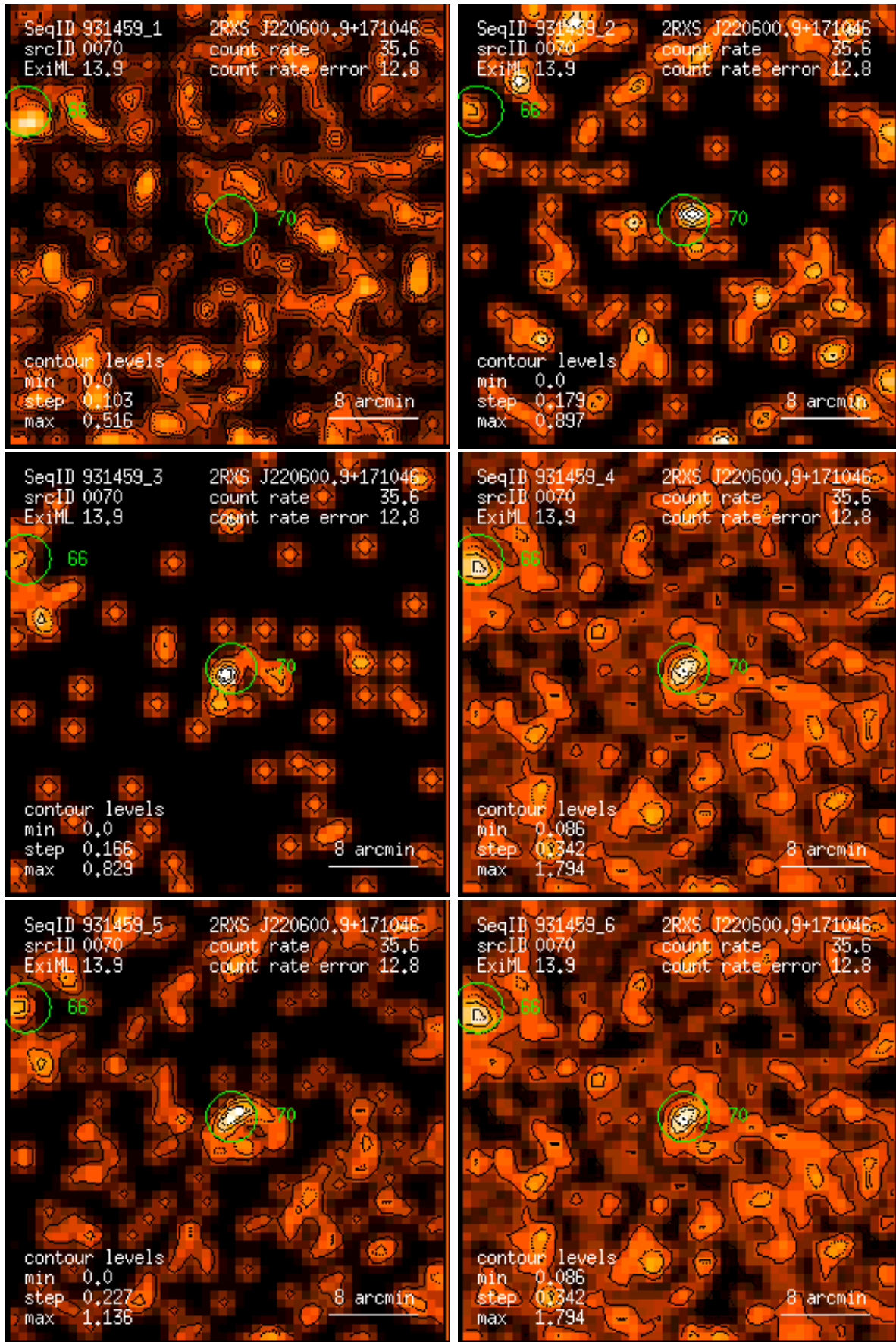
Figure 70: RASS 931459: detection 0070: band rate images, Gaussian filter: (1) PSPC channels 11 – 41, (2) 52 – 90, (3) 91 – 201, (4) 11 – 235, (5) 52 – 201, (6) 11 – 201. Broad band rates in counts/ks. Band rate contour levels in counts/ks/arcmin 2 .
