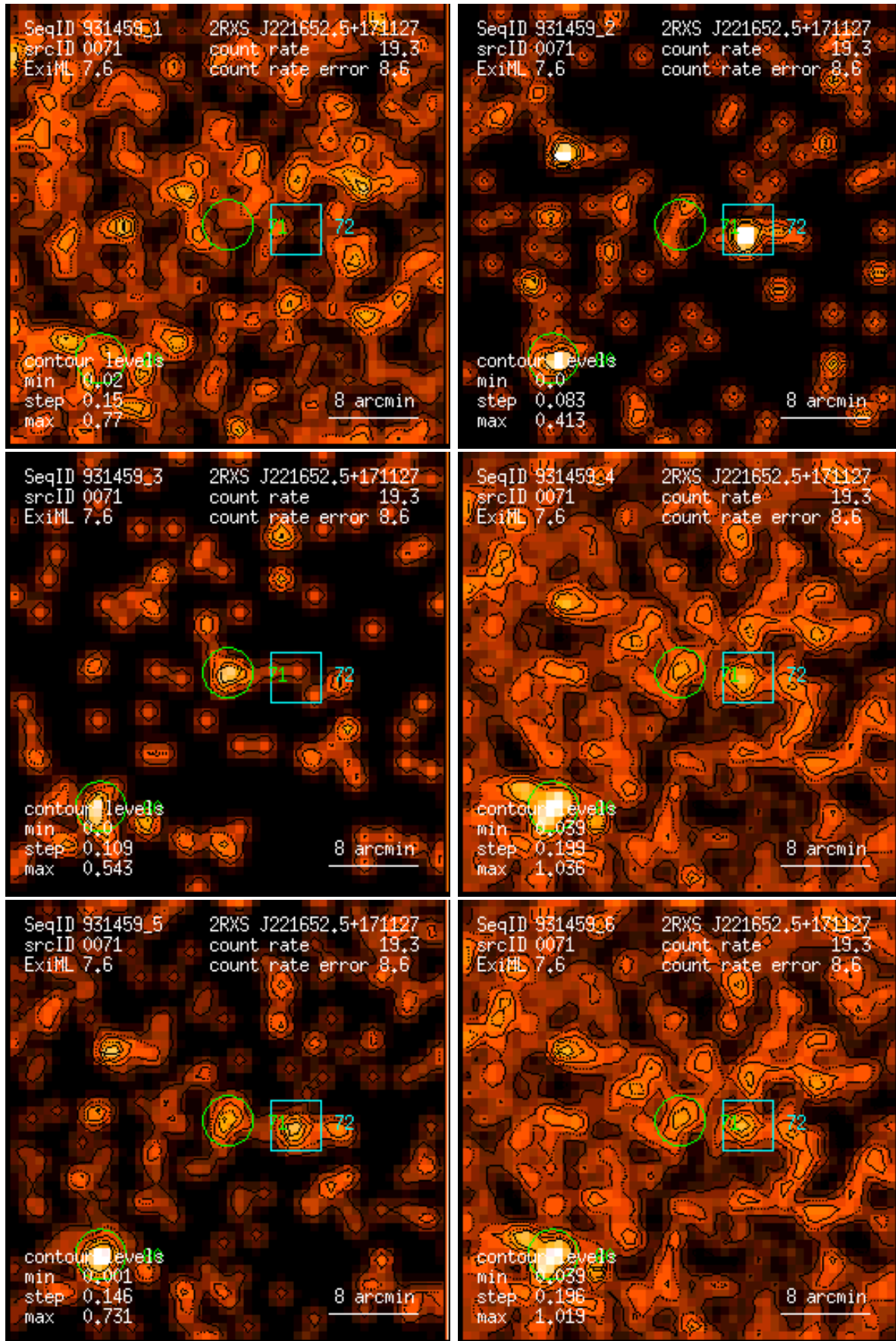
Figure 71: RASS 931459: detection 0071: band rate images, Gaussian filter: (1) PSPC channels 11 – 41, (2) 52 – 90, (3) 91 – 201, (4) 11 – 235, (5) 52 – 201, (6) 11 – 201. Broad band rates in counts/ks. Band rate contour levels in counts/ks/arcmin 2 .
