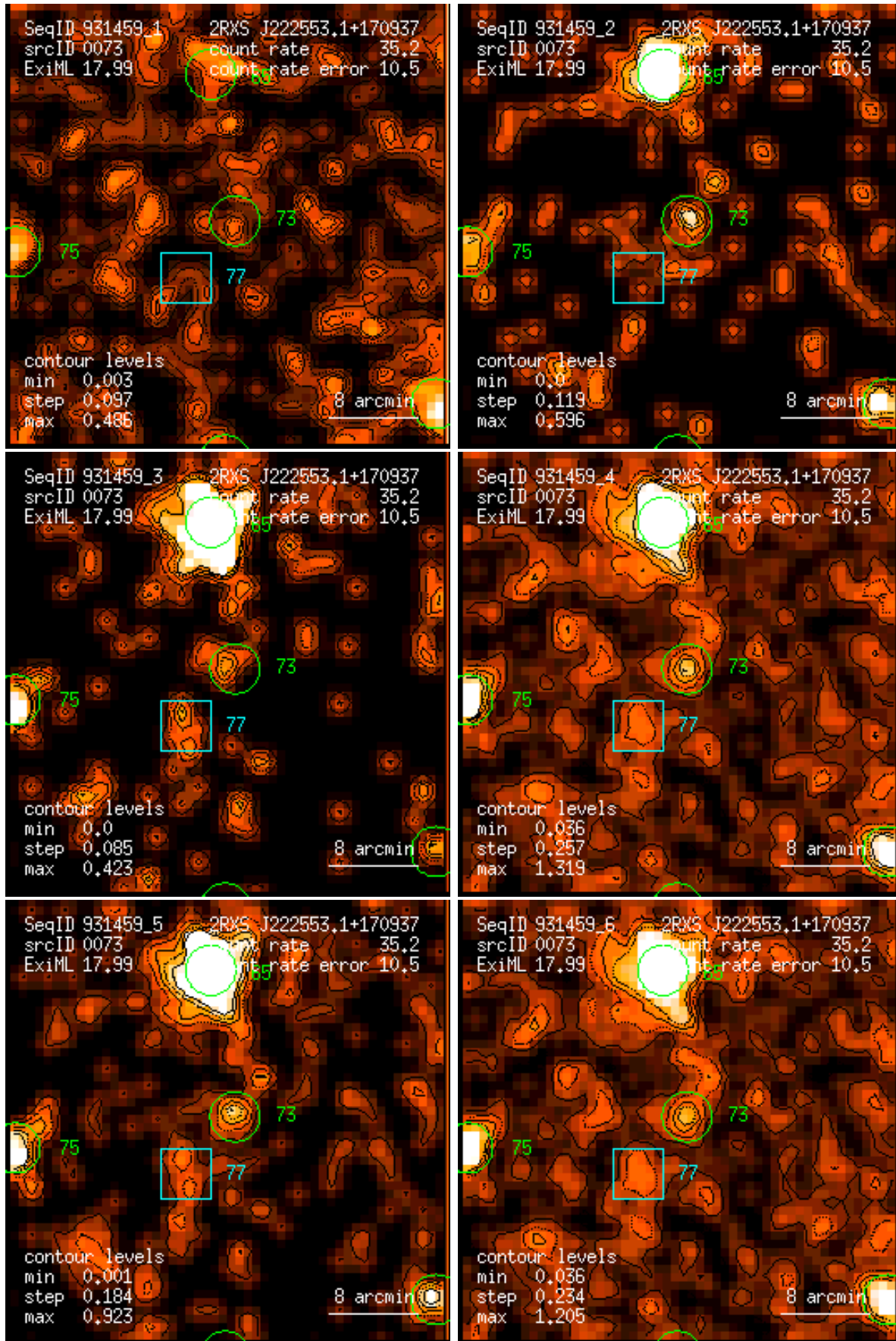
Figure 73: RASS 931459: detection 0073: band rate images, Gaussian filter: (1) PSPC channels 11 – 41, (2) 52 – 90, (3) 91 – 201, (4) 11 – 235, (5) 52 – 201, (6) 11 – 201. Broad band rates in counts/ks. Band rate contour levels in counts/ks/arcmin 2 .
