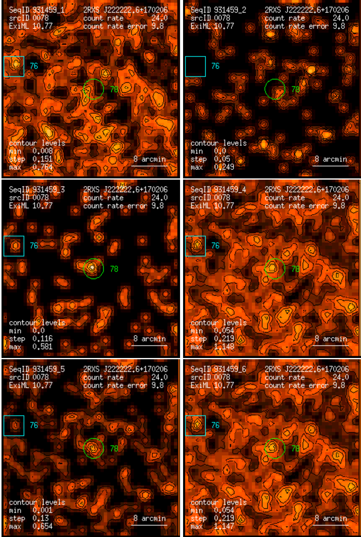
Figure 78: RASS 931459: detection 0078: band rate images, Gaussian filter: (1) PSPC channels 11 – 41, (2) 52 – 90, (3) 91 – 201, (4) 11 – 235, (5) 52 – 201, (6) 11 – 201. Broad band rates in counts/ks. Band rate contour levels in counts/ks/arcmin 2 .
