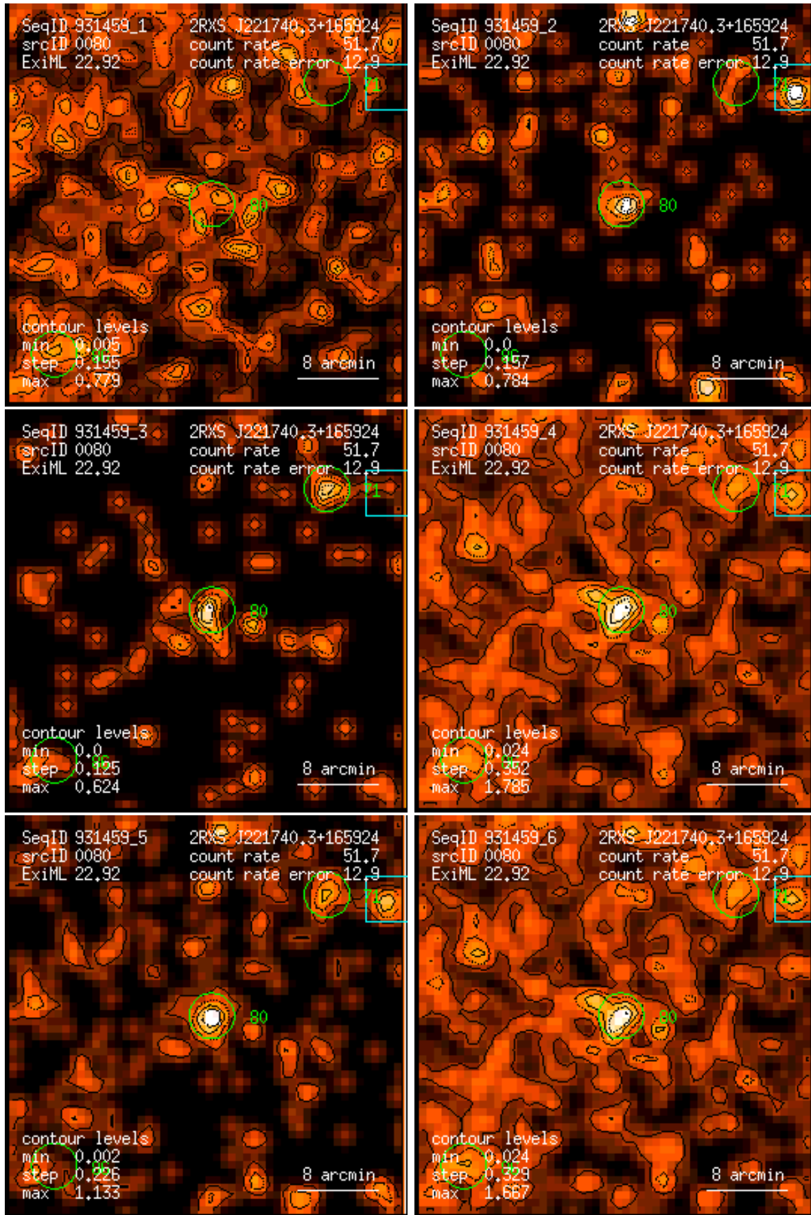
Figure 80: RASS 931459: detection 0080: band rate images, Gaussian filter: (1) PSPC channels 11 – 41, (2) 52 – 90, (3) 91 – 201, (4) 11 – 235, (5) 52 – 201, (6) 11 – 201. Broad band rates in counts/ks. Band rate contour levels in counts/ks/arcmin 2 .
