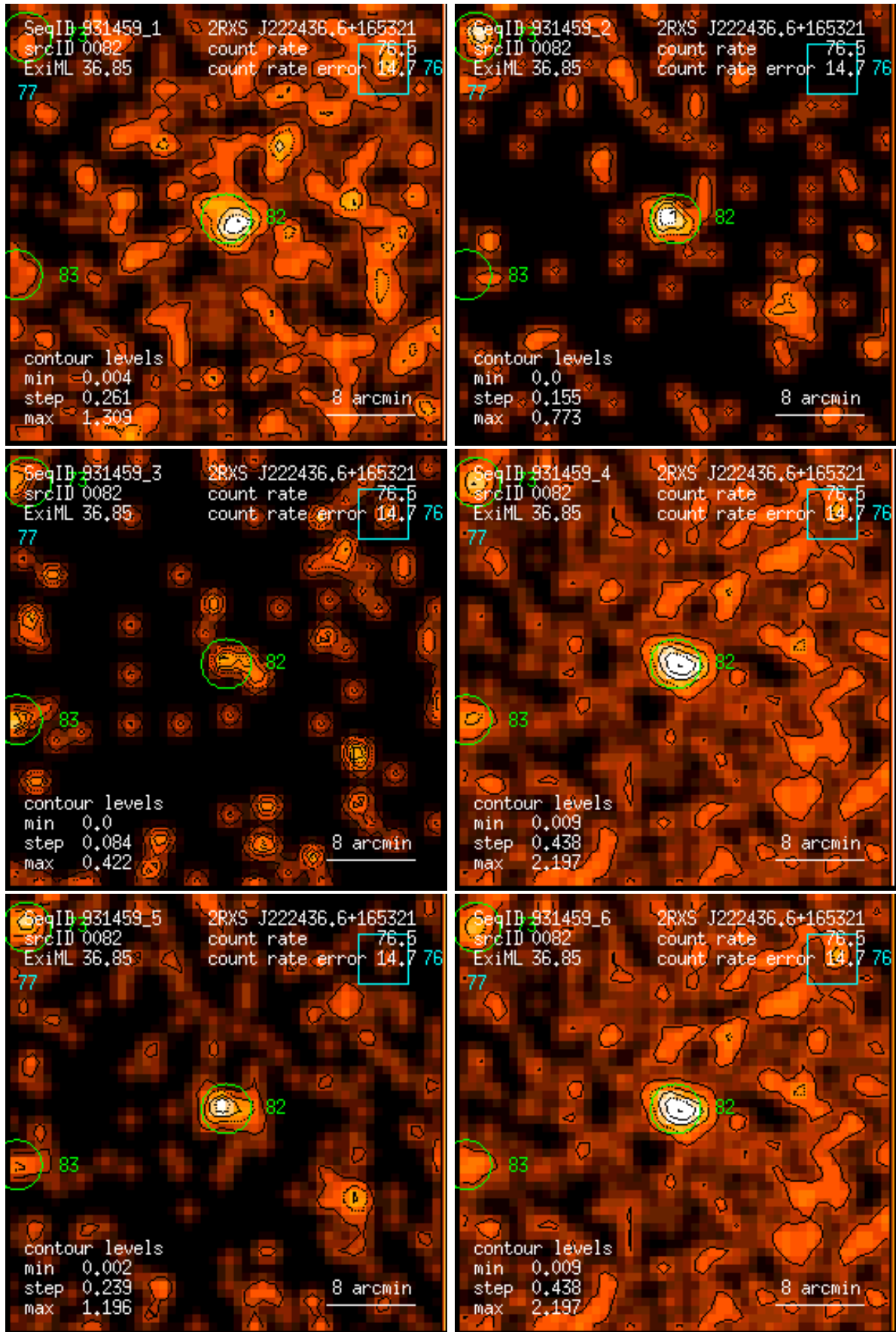
Figure 82: RASS 931459: detection 0082: band rate images, Gaussian filter: (1) PSPC channels 11 – 41, (2) 52 – 90, (3) 91 – 201, (4) 11 – 235, (5) 52 – 201, (6) 11 – 201. Broad band rates in counts/ks. Band rate contour levels in counts/ks/arcmin 2 .
